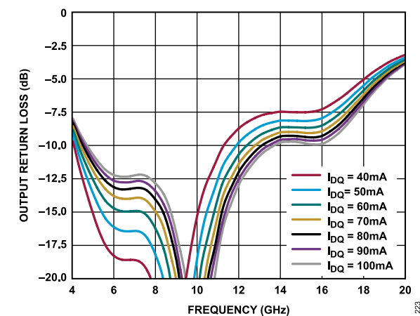
Figure 23. Output Return Loss vs. Frequency for Various I_{DQ} , V_{DD} = 5\text{ V}
