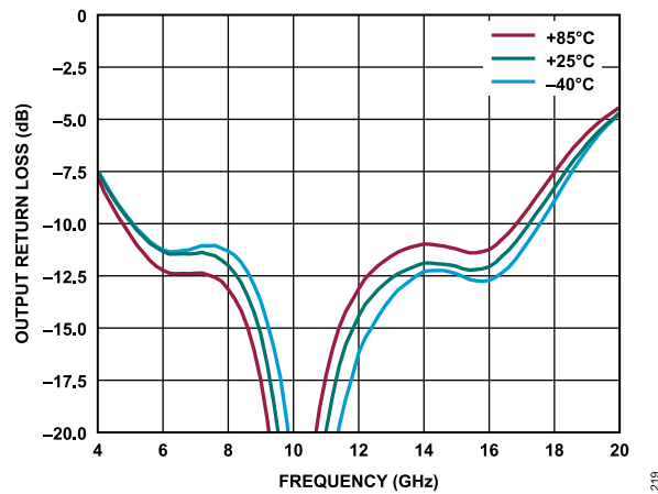
Figure 19. Output Return Loss vs. Frequency for Various Temperatures, 4 GHz to 20 GHz, V_{DD} = 3\text{ V} , I_{DQ} = 90\text{ mA} , R_{BIAS} = 2.7\text{ k}\Omega
