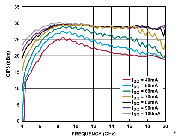
Figure 59. OIP3 vs. Frequency for Various I_{DQ} , V_{DD} = 5\text{ V}
