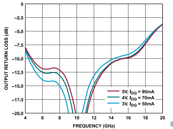
Figure 20. Output Return Loss vs. Frequency for Various Supply Voltages and I_{DQ} , R_{BIAS} = 7.15\text{ k}\Omega
