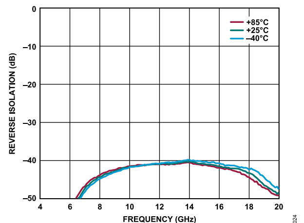
Figure 24. Reverse Isolation vs. Frequency for Various Temperatures, 4 GHz to 20 GHz, V_{DD} = 5\text{ V} , I_{DQ} = 90\text{ mA} , R_{BIAS} = 7.15\text{ k}\Omega
