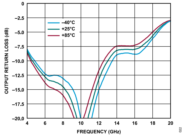
Figure 22. Output Return Loss vs. Frequency for Various Temperatures, 4 GHz to 20 GHz, V_{DD} = 5\text{ V} , I_{DQ} = 90\text{ mA} , R_{BIAS} = 7.15\text{ k}\Omega
