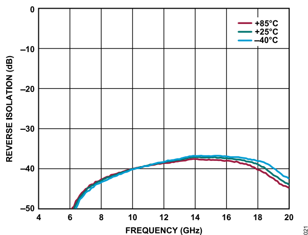
Figure 21. Reverse Isolation vs. Frequency for Various Temperatures, 4 GHz to 20 GHz, V_{DD} = 3\text{ V} , I_{DQ} = 90\text{ mA} , R_{BIAS} = 2.7\text{ k}\Omega
