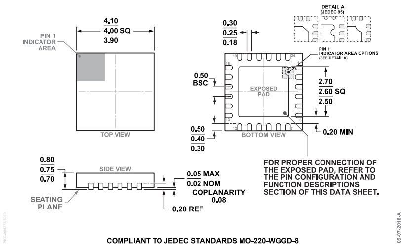
Figure 56. 24-Lead Lead Frame Chip Scale Package [LFCSP] 4 mm x 4 mm Body and 0.75 mm Package Height (CP-24-15) Dimensions shown in millimeters
