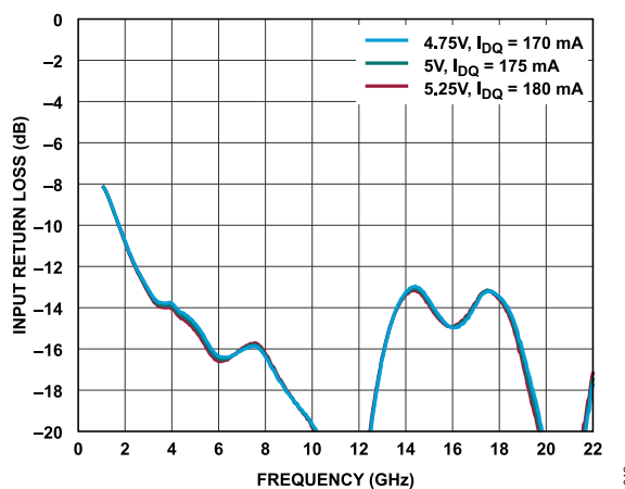
Figure 12. Input Return Loss vs. Frequency for Various V_{DD} and I_{DQ} Values, R_{BIAS} = 698\ \Omega
