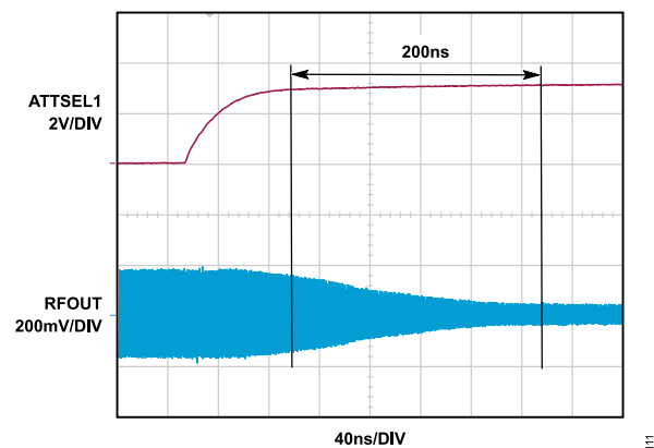
Figure 11. Gain Settling Time at DSA1 = 0.00 dB (Minimum), DSA2 from 0.00 dB to 15.75 dB
