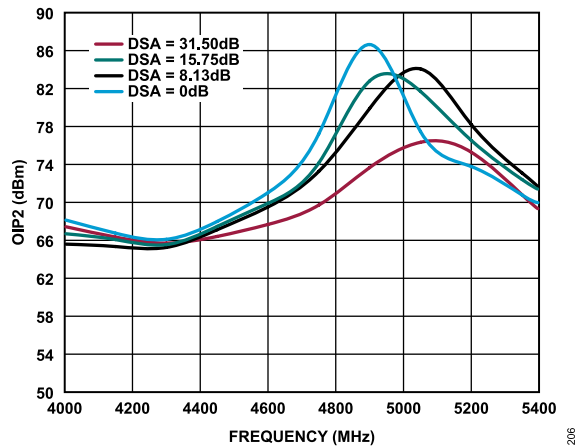
Figure 106. OIP2 vs. Frequency at Various DSA Values
