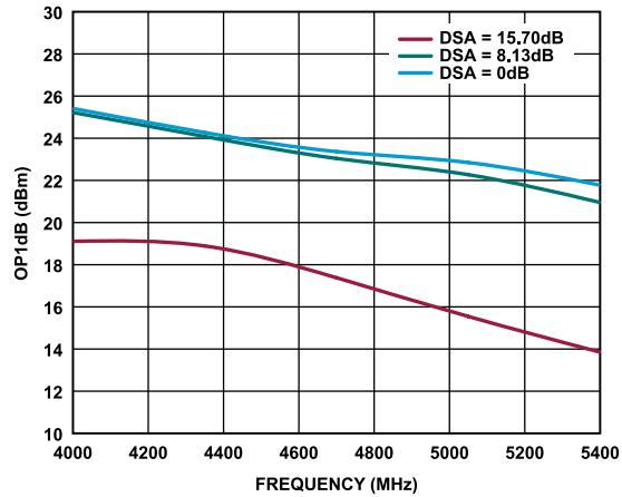
Figure 99. OP1dB vs. Frequency at Various DSA Values
