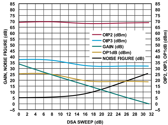
Figure 85. Gain, Noise Figure, OIP2, OIP3, OP1dB vs. DSA Sweep, Frequency = 3600 MHz
