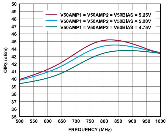
Figure 19. OIP3 vs. Frequency for Various Supplies
