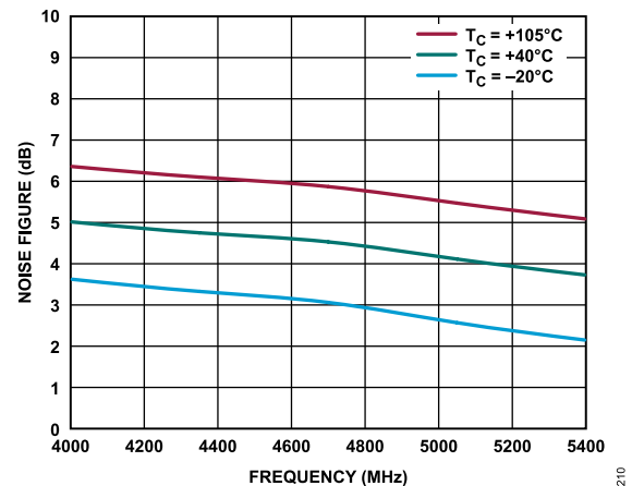
Figure 110. Noise Figure vs. Frequency for Various Temperatures
