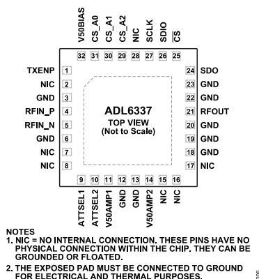
Figure 6. Pin Configuration
