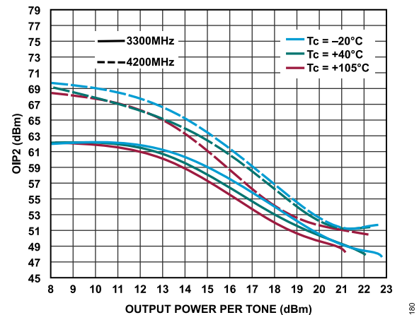
Figure 80. OIP2 vs. Output Power per Tone for Various Temperatures at 3300 MHz and 4200 MHz
