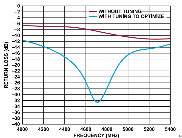
Figure 117. Return Loss of Differential RF Input S11 at 100 \Omega Match; 0.6 pF in Shunt and 0.8 nH Series on Each Input
