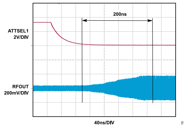
Figure 10. Gain Settling Time at DSA1 = 0.00 dB (Minimum), DSA2 from 15.75 dB to 0.00 dB
