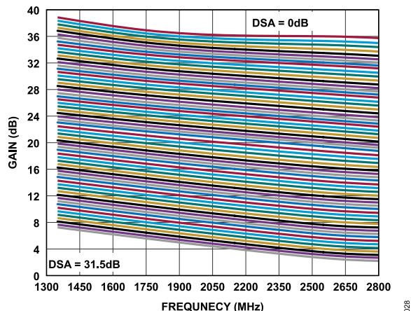
Figure 39. Gain vs. Frequency; 0.5 dB DSA Steps
