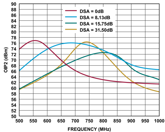
Figure 25. OIP2 vs. Frequency at Various DSA Values
