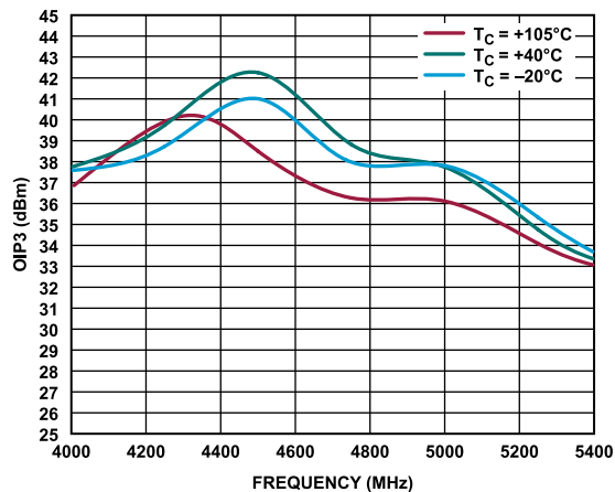
Figure 101. OIP3 vs. Frequency for Various Temperatures
