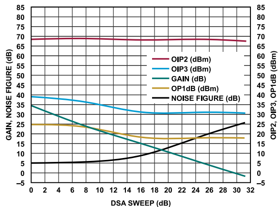
Figure 86. Gain, Noise Figure, OIP2, OIP3, OP1dB vs. DSA Sweep, Frequency = 4200 MHz
