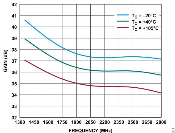
Figure 41. Gain vs. Frequency for Various Temperatures
