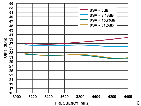
Figure 75. OIP3 vs. Frequency at Various DSA Values
