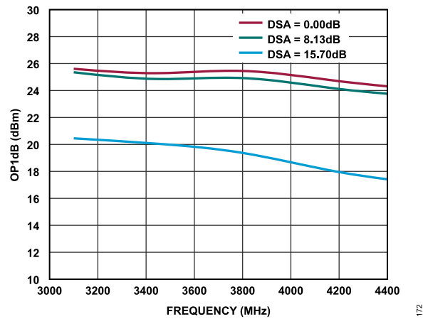
Figure 72. OP1dB vs. Frequency at Various DSA Values
