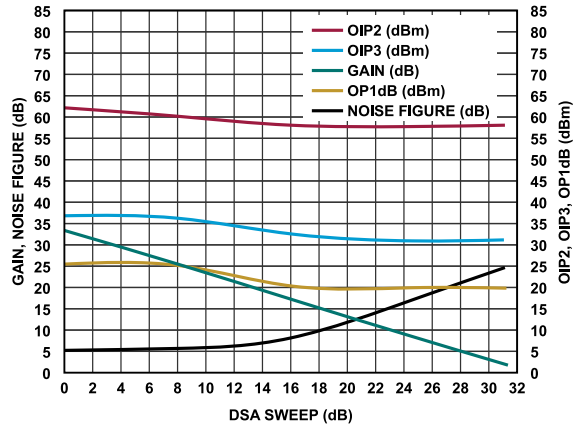
Figure 84. Gain, Noise Figure, OIP2, OIP3, OP1dB vs. DSA Sweep, Frequency = 3300 MHz
