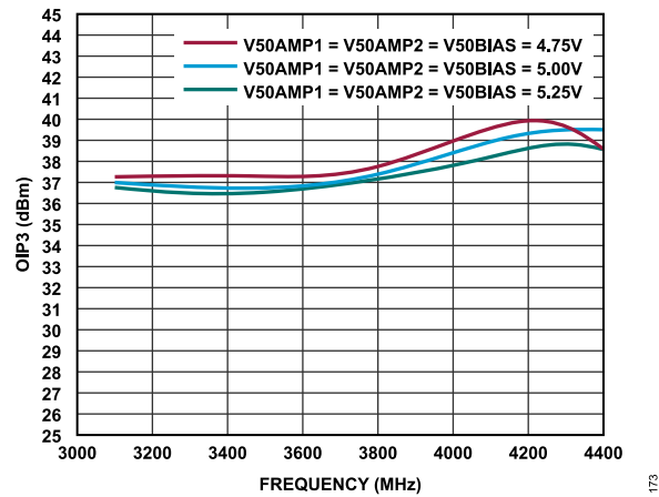
Figure 73. OIP3 vs. Frequency for Various Supplies
