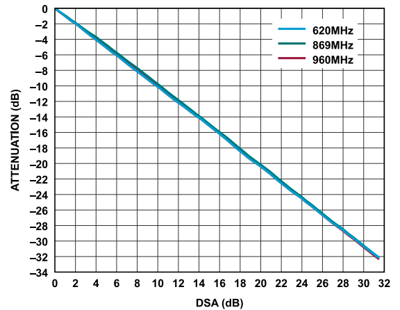
Figure 15. Attenuation vs. DSA at 620 MHz, 869 MHz, and 960 MHz
