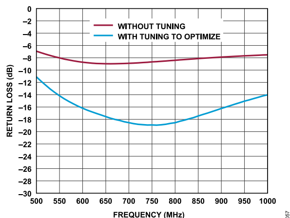
Figure 36. Return Loss of Differential RF Input S11 at 100 \Omega Match; 14 nH in Shunt and 30 pF Series on Each Input
