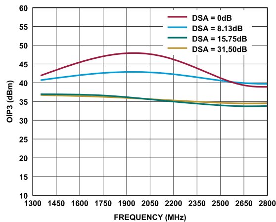
Figure 48. OIP3 vs. Frequency at Various DSA Values
