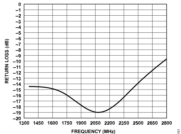
Figure 62. Return Loss of Single-Ended RF Output S22 at 50 \Omega Match
