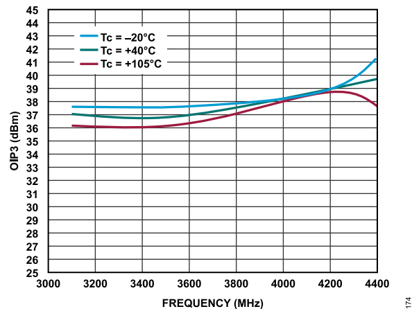
Figure 74. OIP3 vs. Frequency for Various Temperatures
