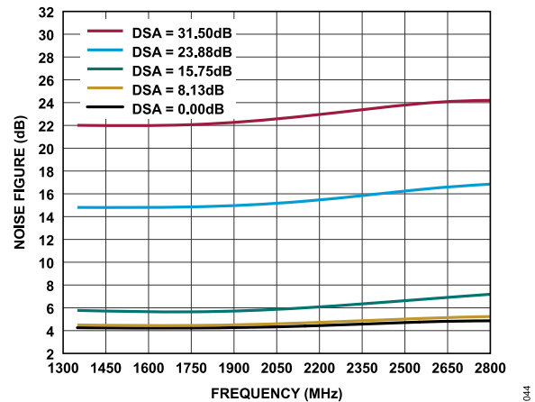
Figure 55. Noise Figure vs. Frequency at Various DSA Values
