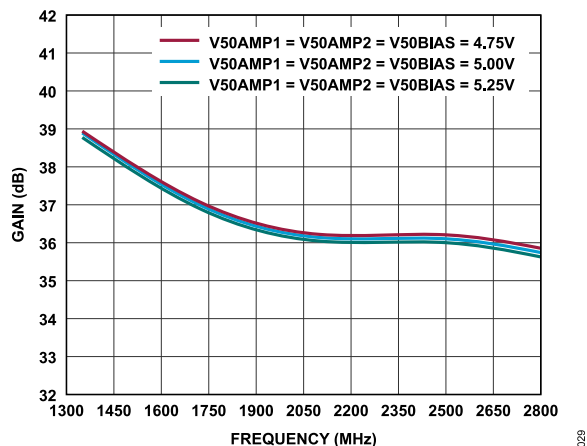
Figure 40. Gain vs. Frequency for Various Supplies
