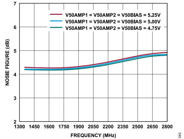
Figure 54. Noise Figure vs. Frequency for Various Supplies
