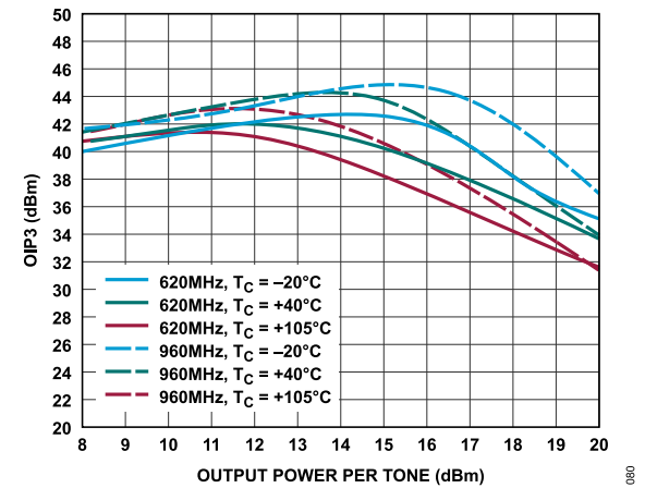
Figure 22. OIP3 vs. Output Power Per Tone for Various Temperatures at 620 MHz and 960 MHz
