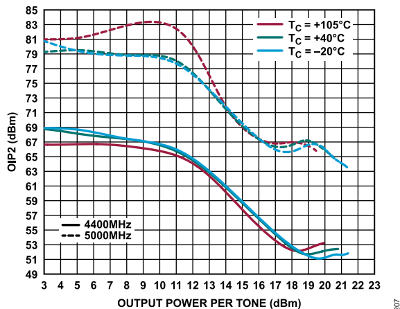
Figure 107. OIP2 vs. Output Power per Tone for Various Temperatures at 4400 MHz and 5000 MHz
