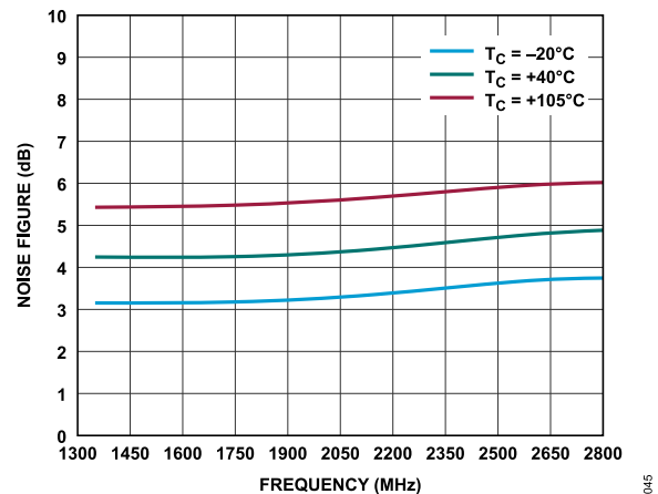
Figure 56. Noise Figure vs. Frequency for Various Temperatures
