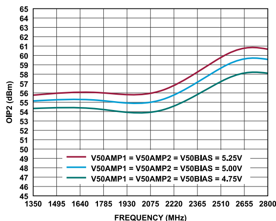
Figure 50. OIP2 vs. Frequency for Various Supplies
