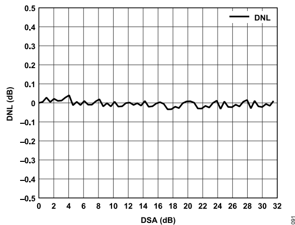
Figure 33. DSA Gain Step Error; Frequency = 869 MHz
