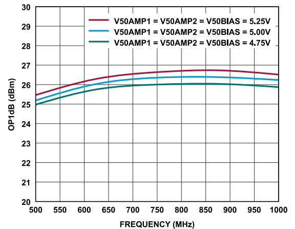
Figure 16. OP1dB vs. Frequency for Various Supplies
