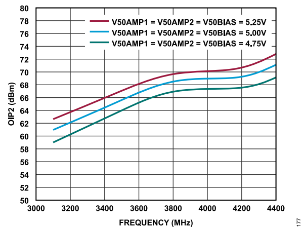
Figure 77. OIP2 vs. Frequency for Various Supplies
