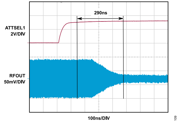
Figure 9. Gain Settling Time at DSA2 = 15.75 dB (Maximum), DSA1 from 0.00 dB to 15.75 dB
