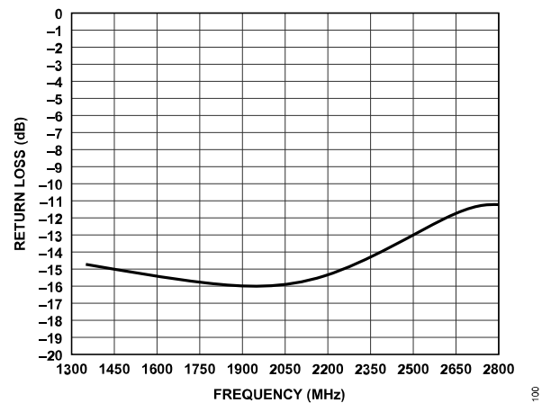
Figure 61. Return Loss of Differential RF Input S11 at 50 \Omega Match
