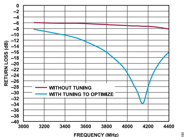
Figure 90. Return Loss of Differential RF Input S11 at 100 \Omega Match; 0.8 pF in Shunt and 1.0 nH Series on Each Input
