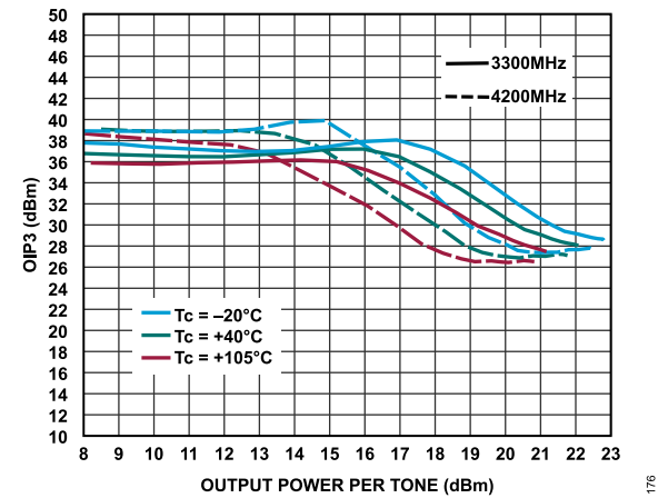
Figure 76. OIP3 vs. Output Power Per Tone for Various Temperatures at 3300 MHz and 4200 MHz
