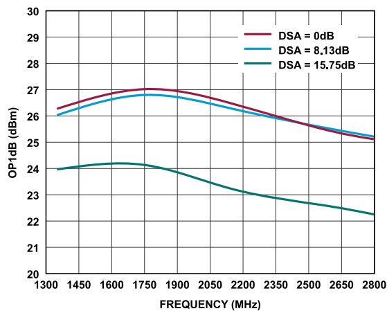
Figure 45. OP1dB vs. Frequency at Various DSA Values
