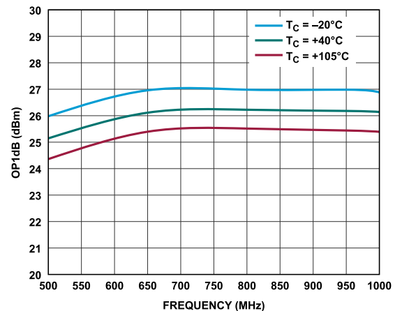
Figure 17. OP1dB vs. Frequency for Various Temperatures
