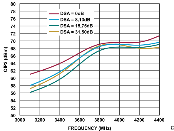
Figure 79. OIP2 vs. Frequency at Various DSA Values
