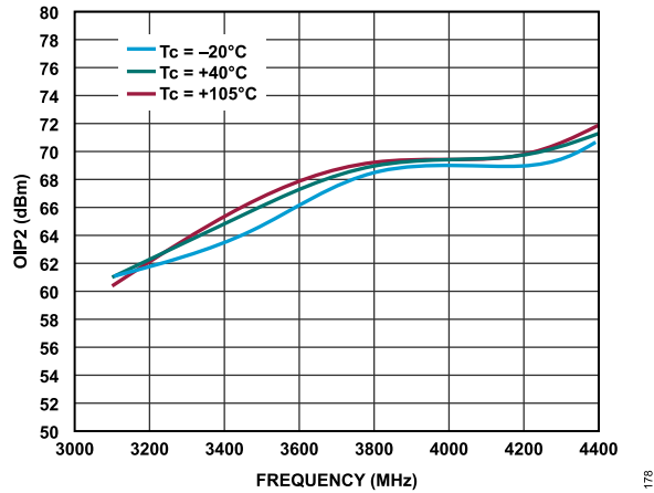
Figure 78. OIP2 vs. Frequency for Various Temperatures
