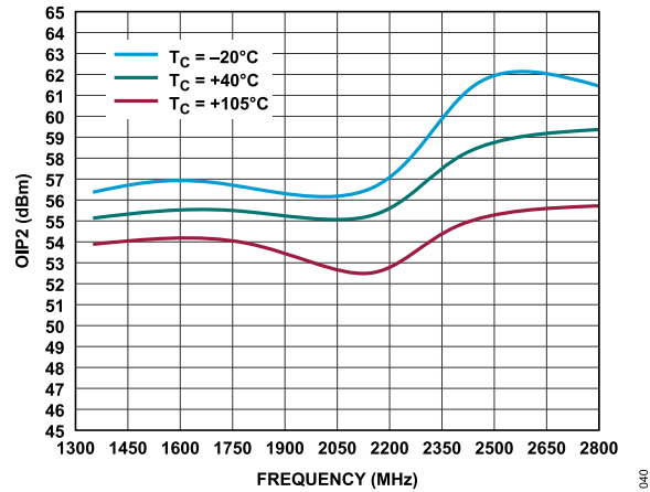
Figure 51. OIP2 vs. Frequency for Various Temperatures
