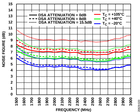
Figure 20. Noise Figure vs. Frequency for Various Temperatures at Various DSA Values, VVA Attenuation = 0 dB
