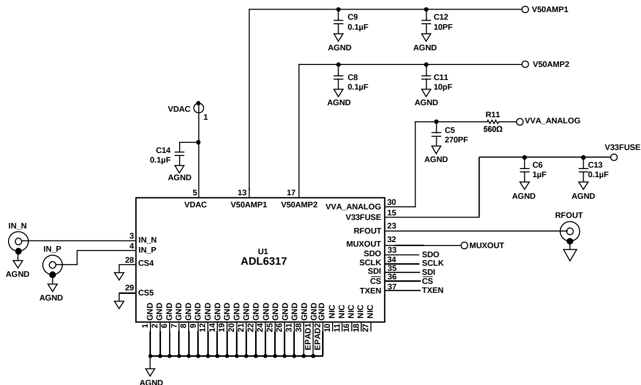
Figure 39. Basic Connections
