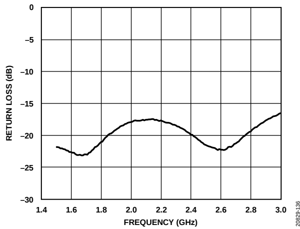
Figure 36. Return Loss of Single-Ended RF Output S22 from 1.5 GHz to 3 GHz
