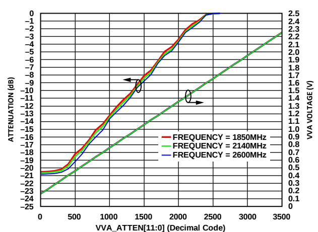
Figure 11. Attenuation and VVA Voltage vs. VVA_ATTEN[11:0] at 1850 MHz, 2150 MHz, and 2600 MHz, DSA Attenuation = 0\text{ dB}
