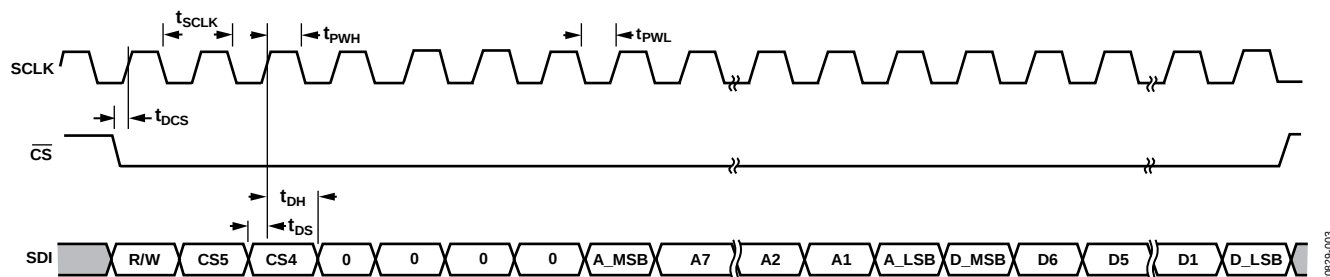
Figure 3. Timing Diagram for the Serial Port Interface Register Write
