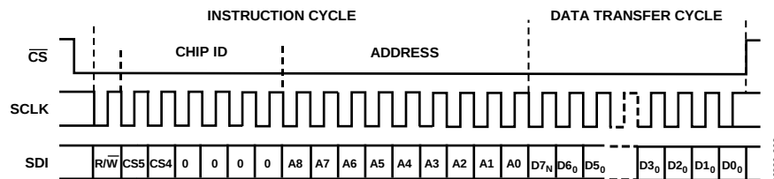
Figure 2. Serial Port Interface Register Timing, MSB First
