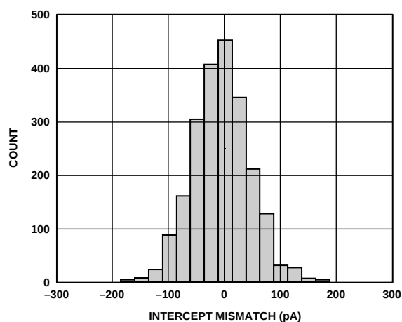
Figure 31. Distribution of Channel-to-Channel Intercept Mismatch ( I_{Z1} - I_{Z2} )
