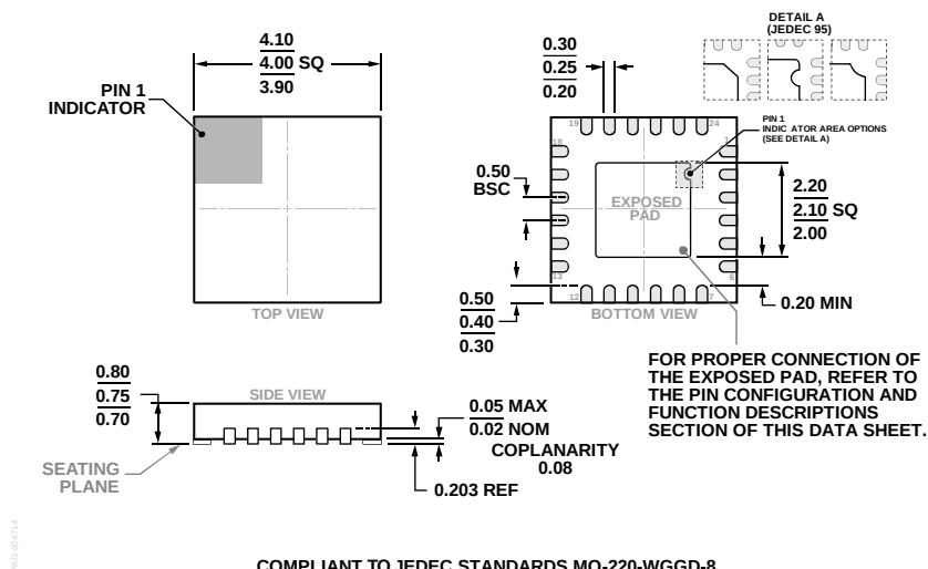
Figure 43. 24-Lead Lead Frame Chip Scale Package [LFCSP] 4 mm × 4 mm Body and 0.75 mm Package Height (CP-24-10)
