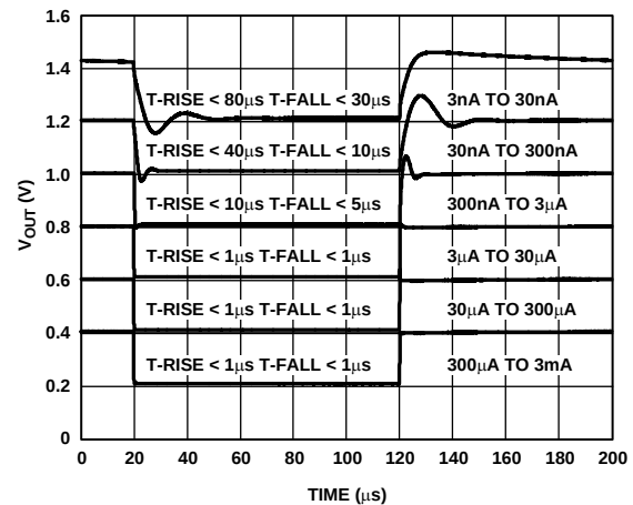
Figure 19. Pulse Response— I_{REF} to V_{OUT} ( A_V = 1 ) in Consecutive 1-Decade Steps
