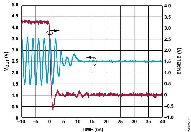
Figure 41. Disable Time Domain Response, 5 V High Performance Mode
