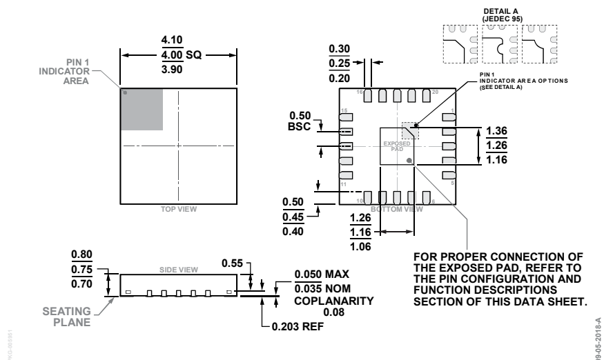
Figure 65. 20-Lead Lead Frame Chip Scale Package [LFCSP] 4 mm x 4 mm Body and 0.75 mm Package Height (CP-20-16) Dimensions shown in millimeters
