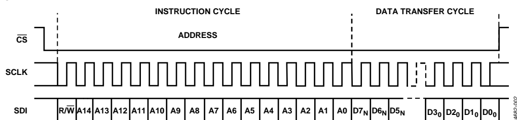
Figure 2. SPI Register Timing, MSB First
