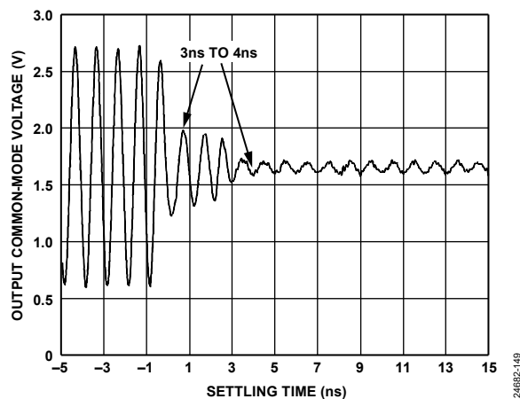
Figure 53. Output Common-Mode Voltage vs. Settling Time, 3.3 V Low Power Mode, Maximum Gain Transition
