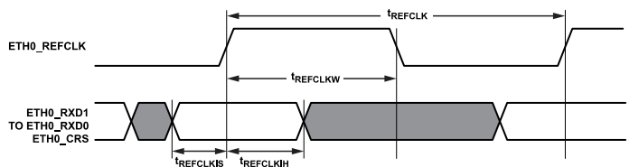
Figure 2. RMII Receive Timing
