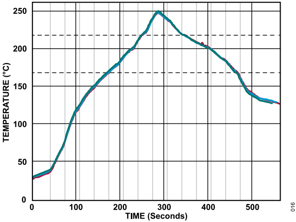
Figure 15. High Peak Reflow Temperature Profile (SMT Process)
