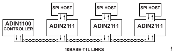
Figure 22. Daisy Chain Topology Using ADIN2111
