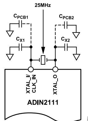
Figure 26. Crystal Oscillator Connection
