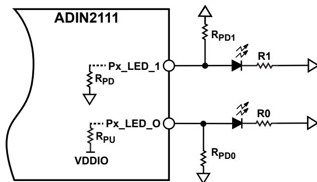
Figure 23. Active High LED Polarity Configuration
