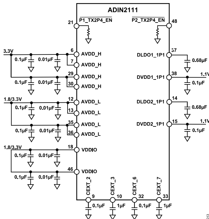
Figure 20. Supplies and Capacitors for Multiple Supply 2.4 V p-p and 1.0 V p-p Transmit Mode
