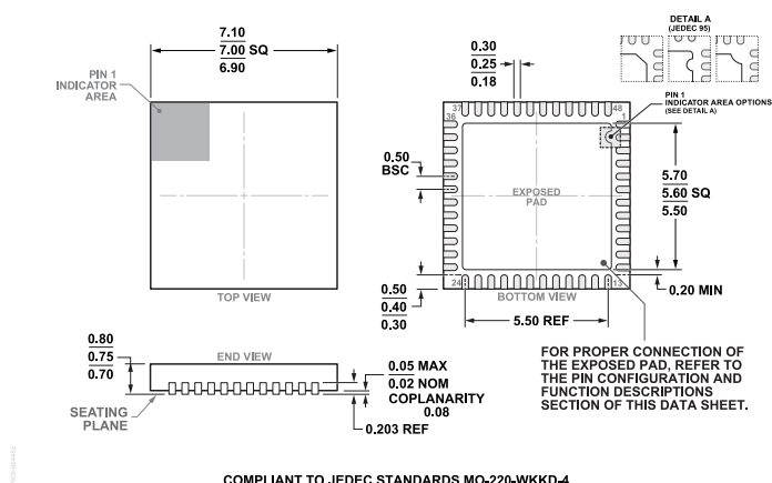
Figure 38. 48-Lead Lead Frame Chip Scale Package [LFCSP] 7 mm × 7 mm Body and 0.75 mm Package Height (CP-48-13) Dimensions shown in millimeters
