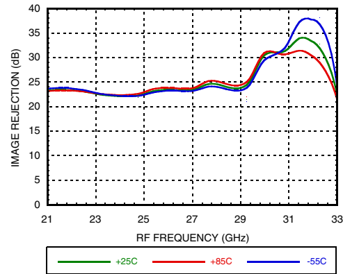
Image Rejection vs. Temperature
