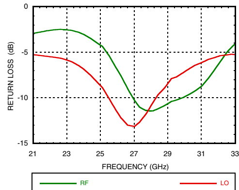
Return Loss
