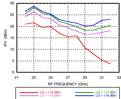
Input IP3 vs. LO Drive
