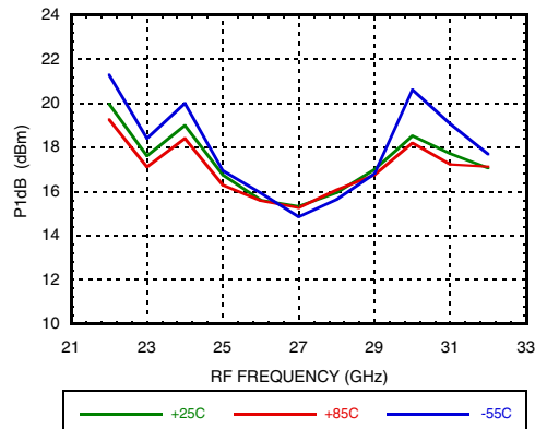
Input P1dB vs. Temperature
