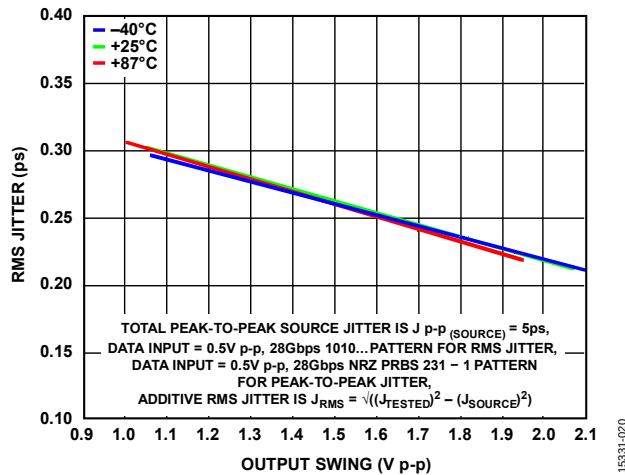
Figure 20. RMS Jitter vs. Output Swing over Temperature, V_{DD} = 5\text{ V} (See Table 3 for Typical Bias Voltages), Total Peak-to-Peak Source Jitter is J_{p-p(SOURCE)} = 5\text{ ps} , Data Input = 0.5 V p-p, 28 Gbps 1010 ... Pattern for RMS Jitter, Data Input = 0.5 V p-p, 28 Gbps NRZ PRBS 2^{31} - 1 Pattern for Peak-To-Peak Jitter, Additive RMS Jitter is J_{RMS} = \sqrt{((J_{TESTED})^2 - (J_{SOURCE})^2)}
