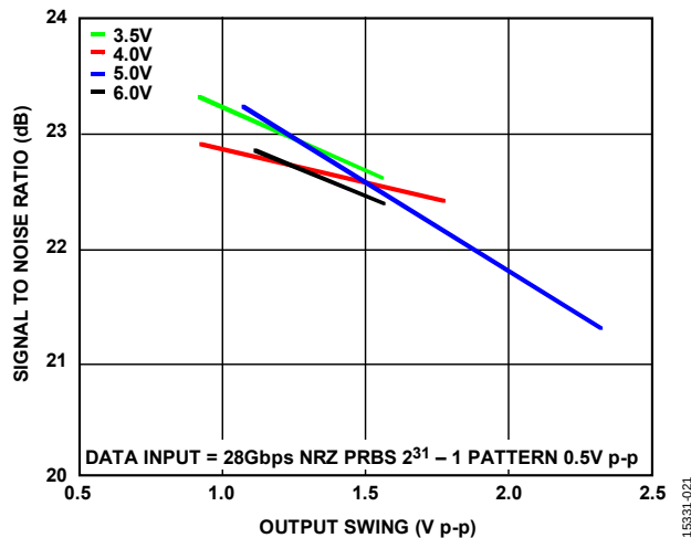
Figure 21. Signal-to-Noise Ratio vs. Output Swing over Supply, V_{GG} = -0.90\text{ V} , Data Input = 28 Gbps NRZ PRBS 2^{31} - 1 Pattern, 0.5 V p-p
