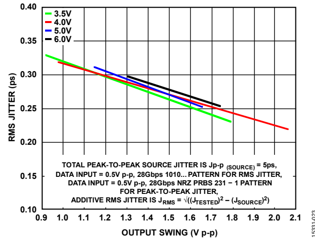
Figure 23. RMS Jitter vs. Output Swing over Supply, V_{GG} = -0.90\text{ V} , Total Peak-to-Peak Source Jitter is J_{p-p(SOURCE)} = 5\text{ ps} , Data Input = 0.5 V p-p, 28 Gbps 1010 ... Pattern for RMS Jitter, Data Input = 0.5 V p-p, 28 Gbps NRZ PRBS 2^{31} - 1 Pattern for Peak-To-Peak Jitter, Additive RMS Jitter is J_{RMS} = \sqrt{((J_{TESTED})^2 - (J_{SOURCE})^2)}
