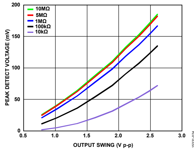
Figure 24. Peak-Detect Voltage vs. Output Swing over R_{LOAD} , V_{DD} = 5\text{ V} (See Table 3 for Typical Bias Voltages), V_{DETBIAS} = 1.2\text{ V} , Peak Detect Voltage = V_{DET} - V_{DETREF} , R_{LOAD} is Equivalent Resistance to GND at V_{DET} and V_{DETREF} Pins
