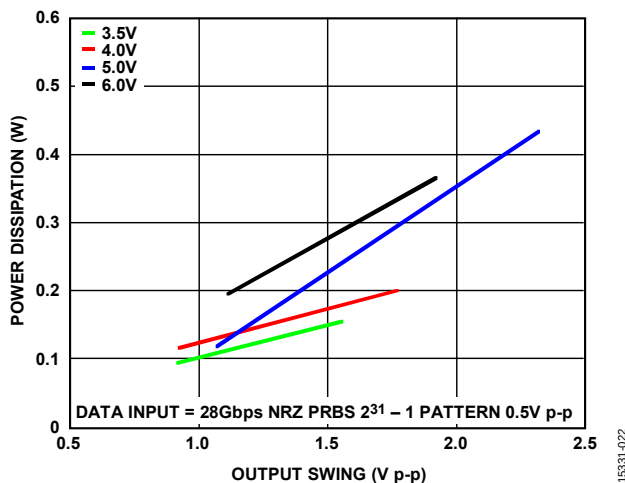
Figure 22. Power Dissipation vs. Output Swing over Supply, V_{GG} = -0.90\text{ V} , Data Input = 28 Gbps NRZ PRBS 2^{31} - 1 Pattern, 0.5 V p-p
