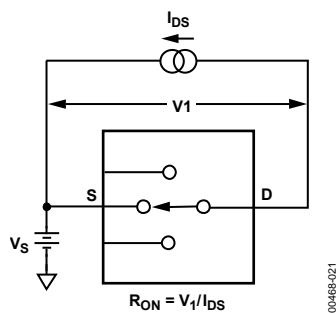
Figure 17. On Resistance
