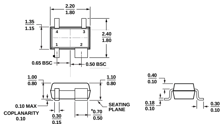
Figure 22. 4-Lead Thin Shrink Small Outline Transistor Package [SC70] (KS-4)
