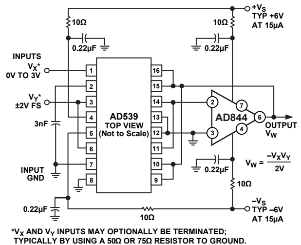
Figure 44. 20 MHz VGA Using the AD539
