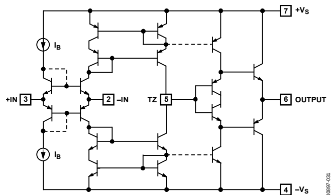
Figure 31. Simplified Schematic
