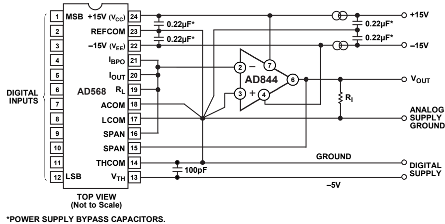
Figure 42. High Speed DAC Amplifier
