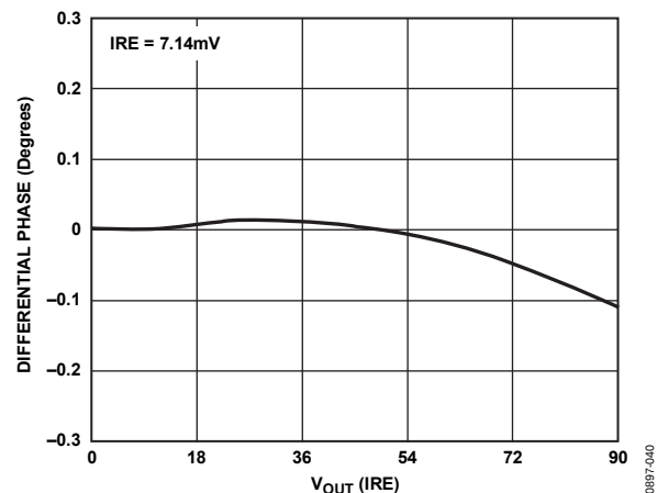
Figure 40. Differential Phase for the Circuit of Figure 38
