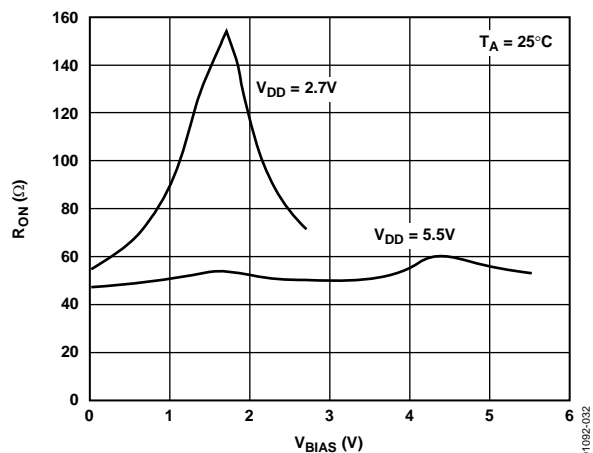
Figure 32. AD8403 Incremental Wiper On Resistance vs. V_{\text{DD}} (See Figure 39)
