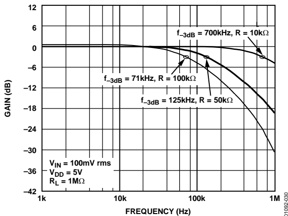
Figure 30. -3\text{ dB} Bandwidths
