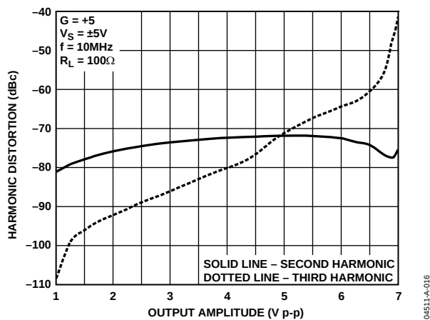
Figure 30. Harmonic Distortion vs. Output Amplitude (SOIC)
