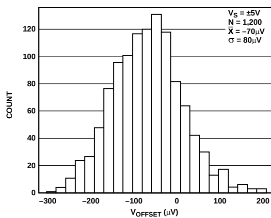
Figure 52. Input Offset Voltage Distribution
