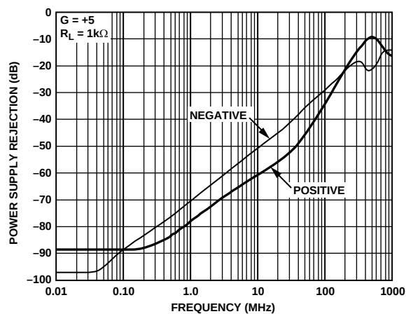
Figure 50. Power Supply Rejection vs. Frequency
