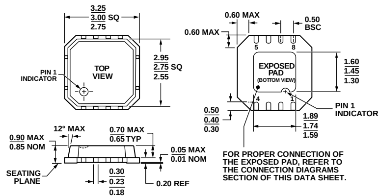
Figure 73. 8-Lead Lead Frame Chip Scale Package [LFCSP_VD] 3 mm × 3 mm Body, Very Thin, Dual Lead (CP-8-2) Dimensions shown in millimeters
