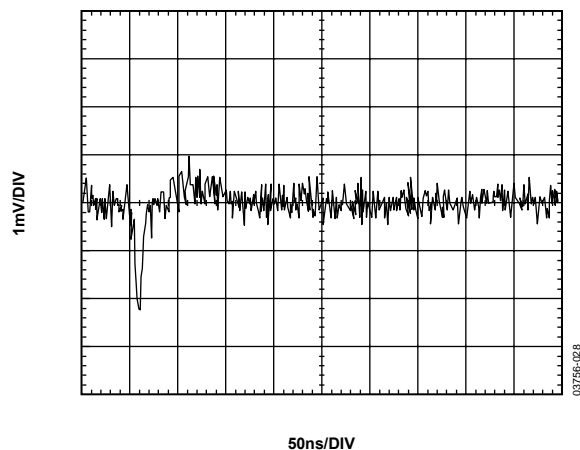
Figure 26. DAC-to-DAC Crosstalk
