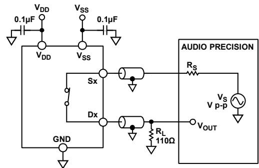
Figure 38. THD + N
