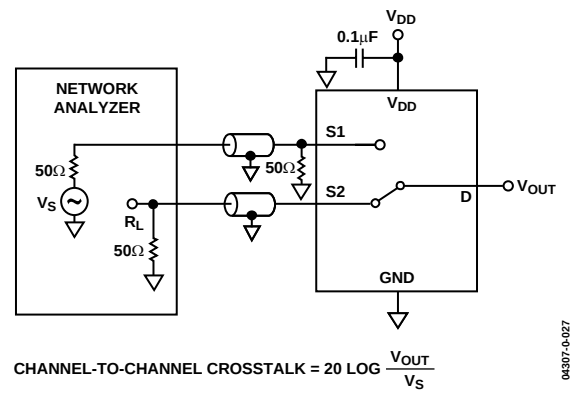
Figure 27. Channel-to-Channel Crosstalk
