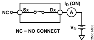
Figure 33. On Leakage
