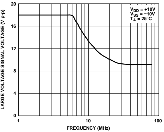
Figure 30. Large Voltage Signal Voltage vs. Frequency
