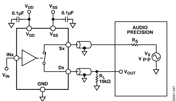
Figure 39. THD + N
