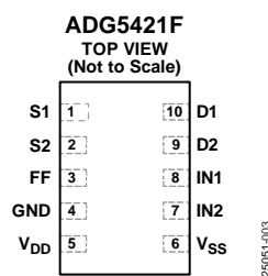
Figure 2. Pin Configuration
