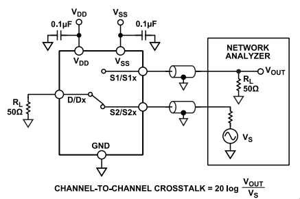
Figure 42. Channel-to-Channel Crosstalk
