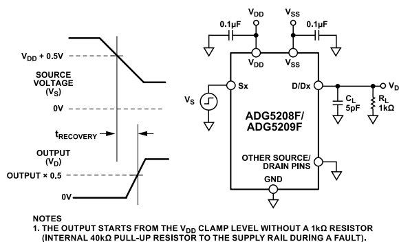
Figure 44. Overvoltage Recovery Time, t_{RECOVERY}
