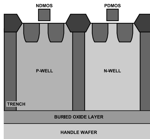
Figure 50. Trench Isolation
