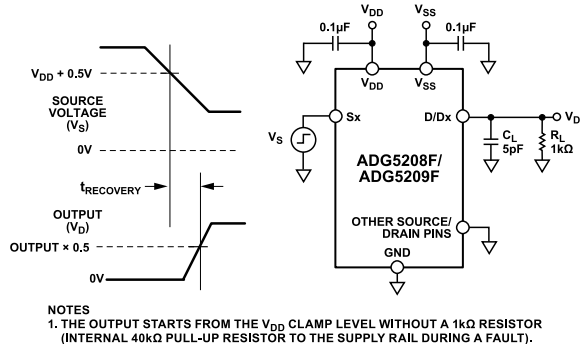
Figure 44. Overvoltage Recovery Time, t_{RECOVERY}
