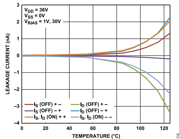
Figure 17. Leakage Current vs. Temperature, 36 V Single Supply
