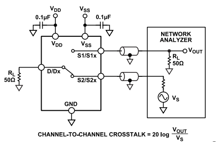
Figure 42. Channel-to-Channel Crosstalk
