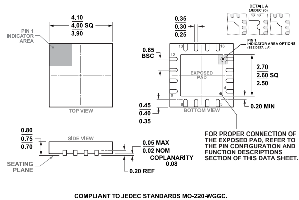
Figure 54. 16-Lead Lead Frame Chip Scale Package [LFCSP] 4 mm × 4 mm Body and 0.75 mm Package Height (CP-16-17) Dimensions shown in millimeters
