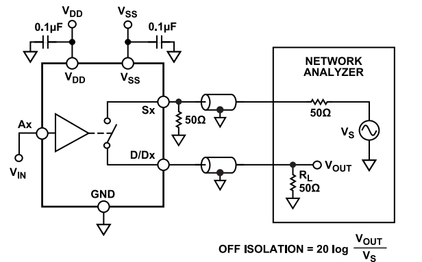
Figure 40. Off Isolation
