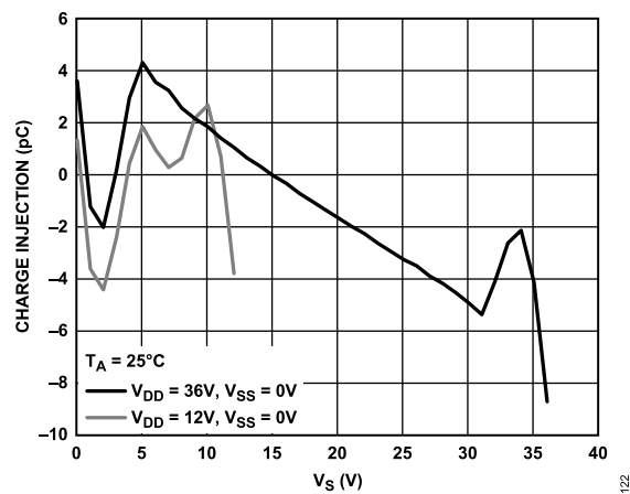
Figure 24. Charge Injection vs. Source Voltage ( V_S ), Single Supply
