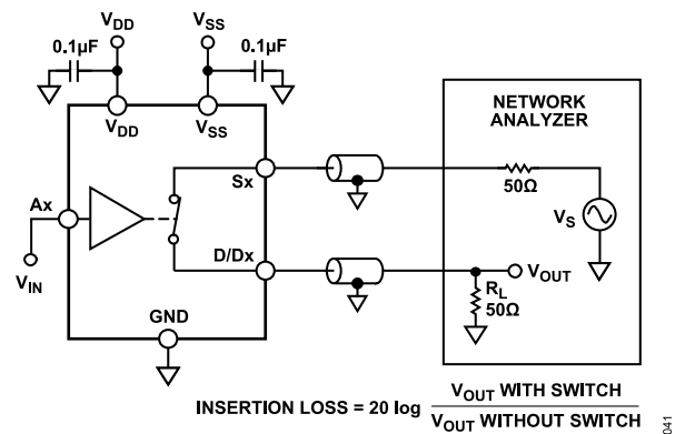
Figure 41. Bandwidth
