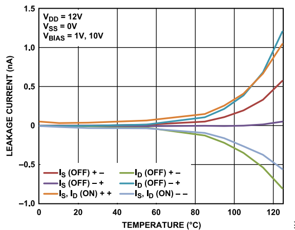
Figure 16. Leakage Current vs. Temperature, 12 V Single Supply
