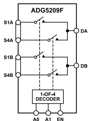
Figure 2. ADG5209F Functional Block Diagram
