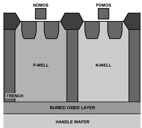
Figure 50. Trench Isolation
