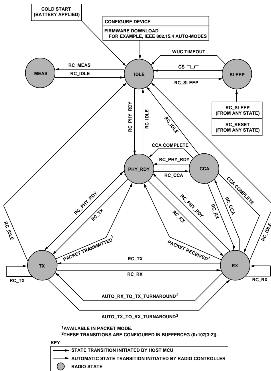
Figure 30. State Diagram
