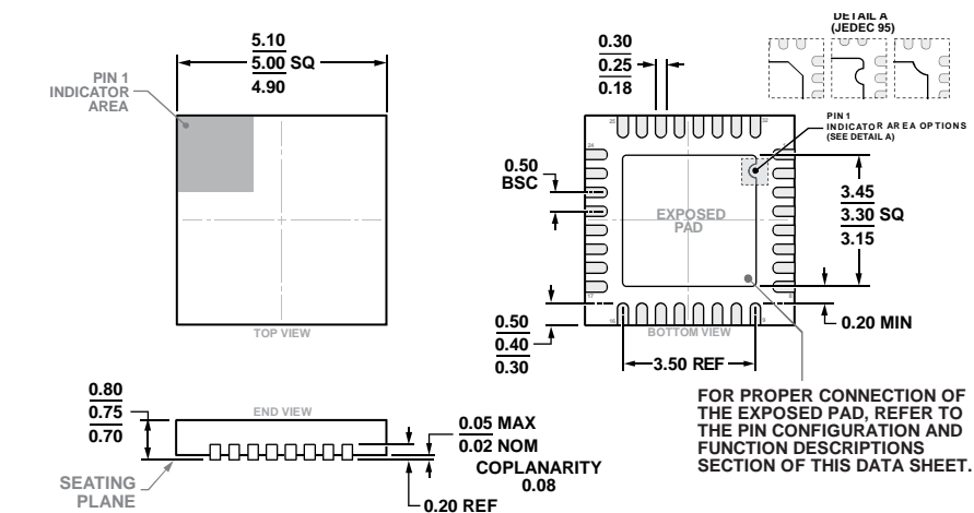
Figure 69. 32-Lead Lead Frame Chip Scale Package [LFCSP] 5 mm x 5 mm Body and 0.75 mm Package Height (CP-32-13)
