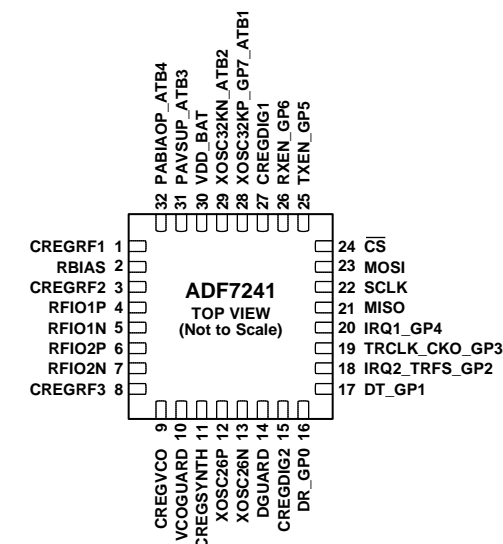
Figure 10. Pin Configuration
