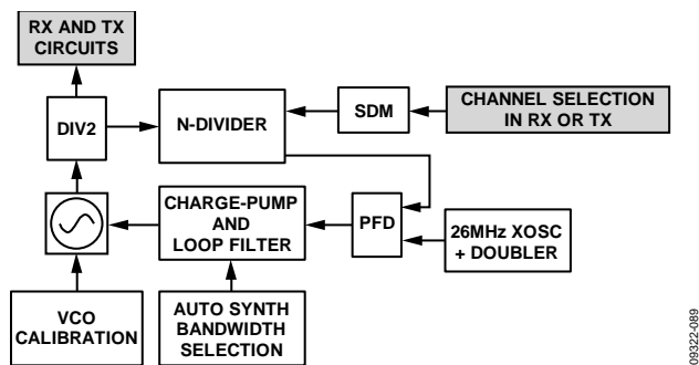
Figure 32. Synthesizer Architecture
