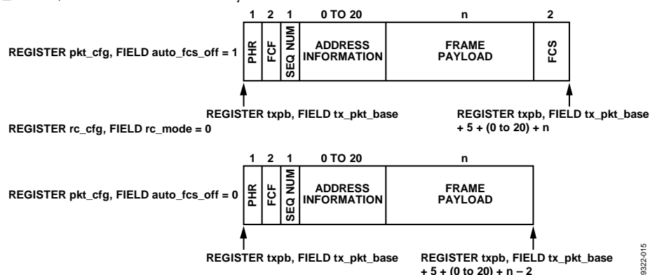
Figure 34. Field Format of TX_BUFFER
