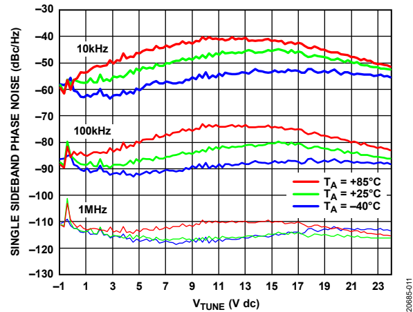
Figure 11. Single Sideband Phase Noise vs. V_{TUNE} for Various Temperatures and Frequencies
