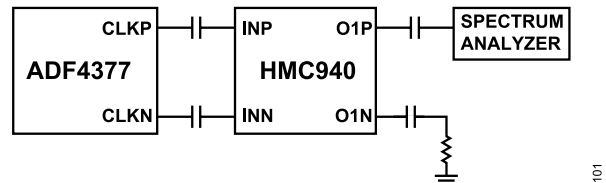
Figure 101. Example of Spurious Measurement Techniques
