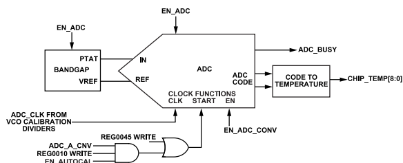
Figure 76. Temperature Sensor
