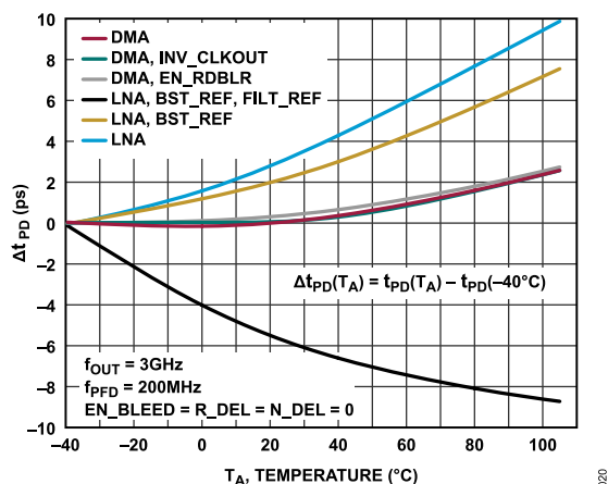
Figure 20. Delta Propagation Delay ( \Delta t_{PD} ) vs. T_A , Temperature, Device Configuration
