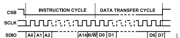
Figure 78. Serial Interface, LSB First (LSB_FIRST = 1)
