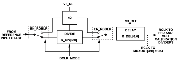
Figure 62. Reference Divider and Doubler
