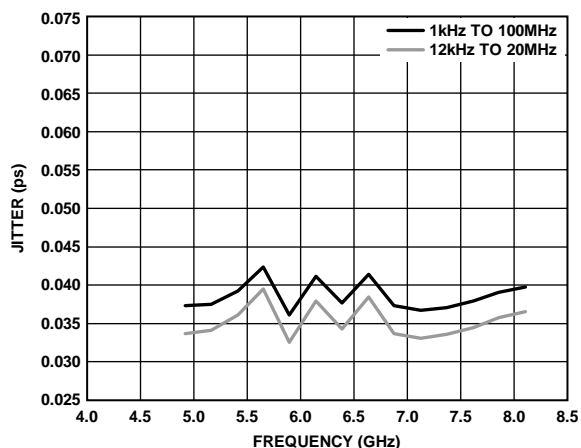
Figure 21. RMS Jitter, Integer-N, f_{PFD} = 245.76 MHz, Loop Filter Bandwidth = 220 kHz, V_{CC\_VCO} = 5 V
