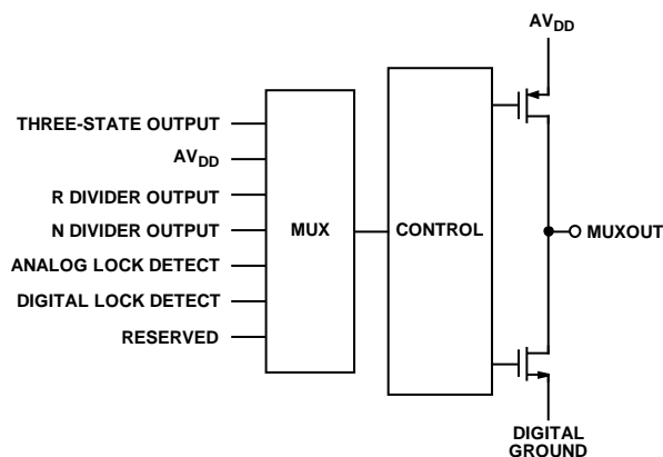
Figure 32. MUXOUT Schematic
