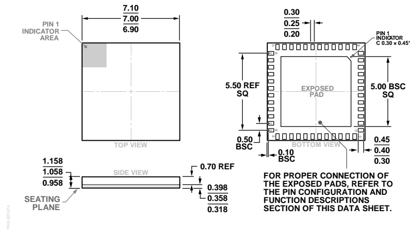
Figure 38. 48-Terminal Land Grid Array [LGA] (CC-48-4) Dimensions shown in millimeters
