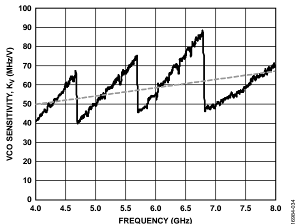
Figure 34. VCO Sensitivity, K_V vs. Frequency, V_{CC\_VCO} = 3.3\text{ V}
