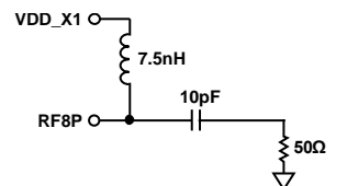
Figure 37. Optimum Output Stage
