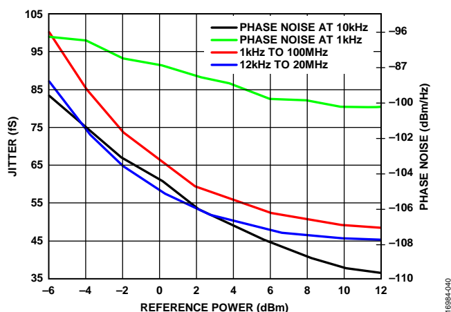
Figure 28. Jitter and Phase Noise, f_{PFD} = 100 MHz
