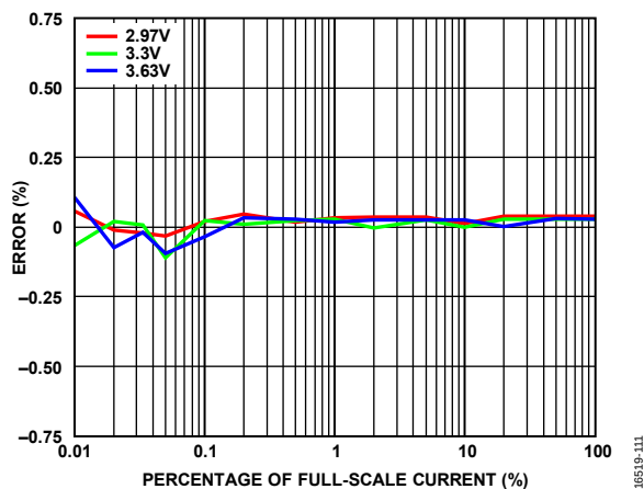
Figure 11. Total Active Energy Error as a Percentage of Full-Scale Current over Supply Voltage, Power Factor = 1, T_A = 25^\circ\text{C} , AI PGA Gain = 38.4x
