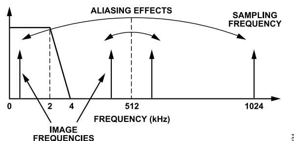
Figure 34. Aliasing Effects
