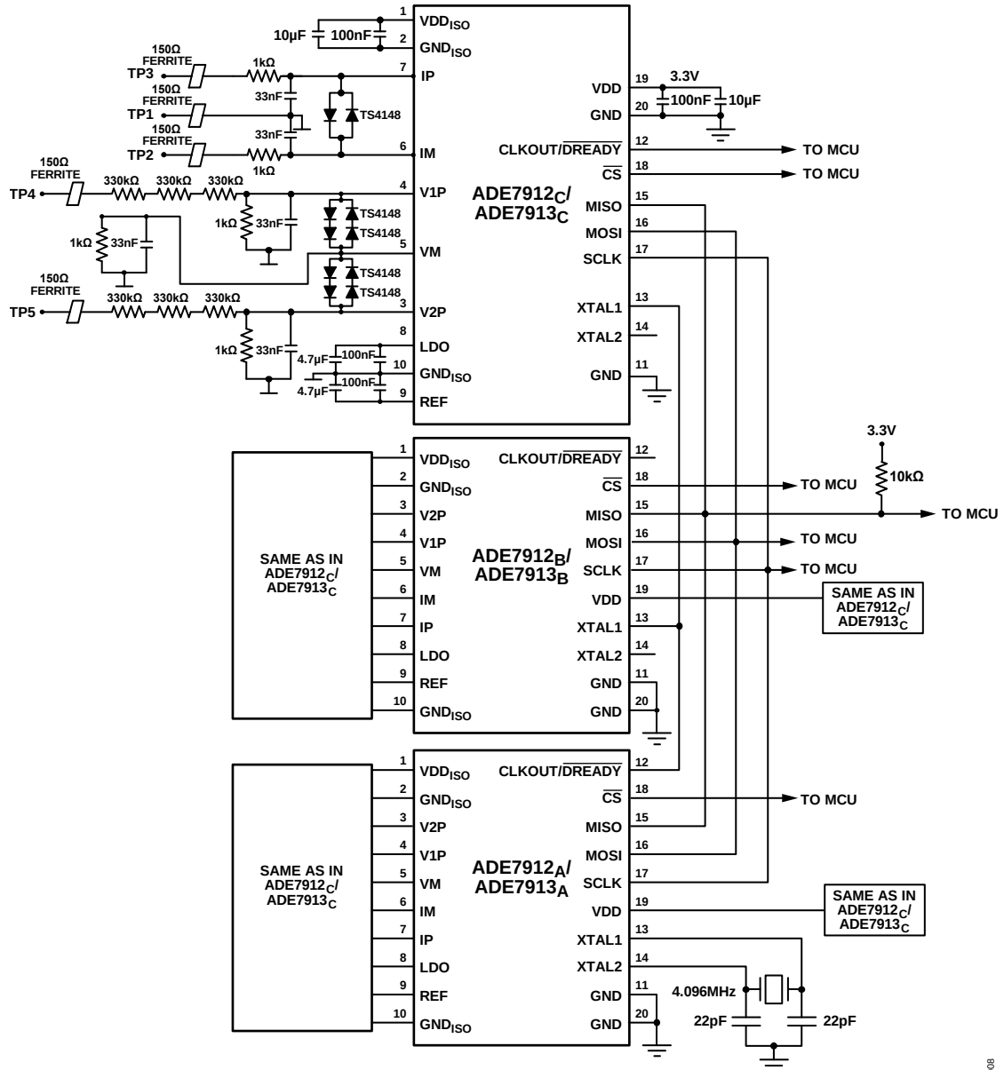
Figure 20. Test Circuit
