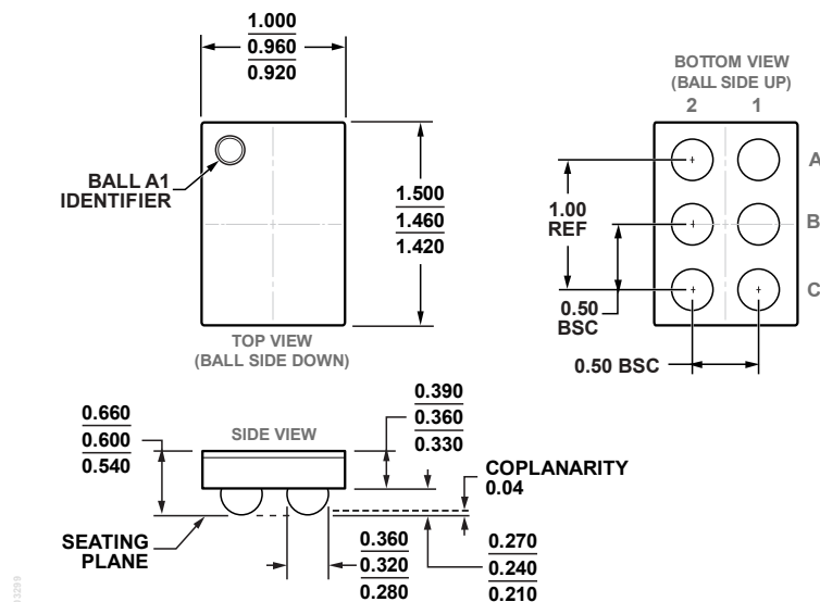
Figure 17. 6-Ball Wafer Level Chip Scale Package [WLCSP] (CB-6-17)
