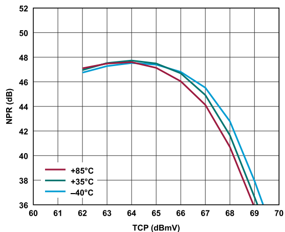
Figure 15. NPR vs. TCP Over Temperature, Worst Case Frequency, 0 dB Tilt, V_{DD} = 8.0 V
