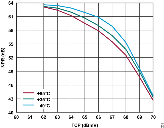
Figure 35. NPR vs. TCP Over Temperature, Worst Case Frequency, 0 dB Tilt, V_{DD} = 8.0\text{ V}
