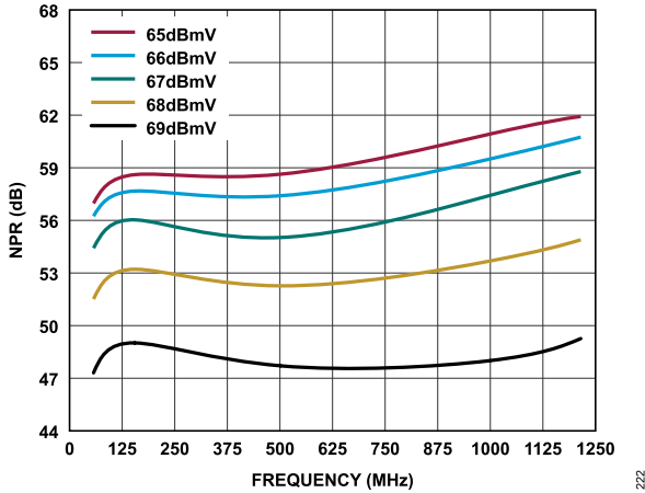
Figure 22. NPR vs. Frequency Over TCP, 10 dB Tilt, V_{DD} = 8.0\text{ V}
