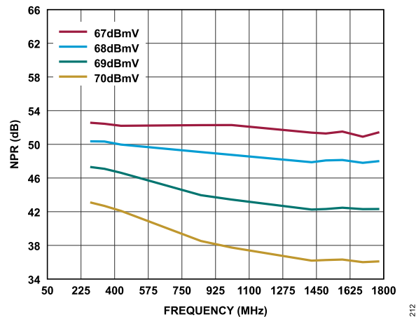
Figure 12. NPR vs. Frequency Over TCP, 10 dB Tilt, No Offset at 1026 MHz, V_{DD} = 8.0\text{ V}
