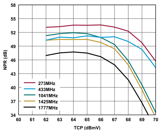
Figure 16. NPR vs. TCP Over Frequency, 0 dB Tilt, V_{DD} = 8.0 V
