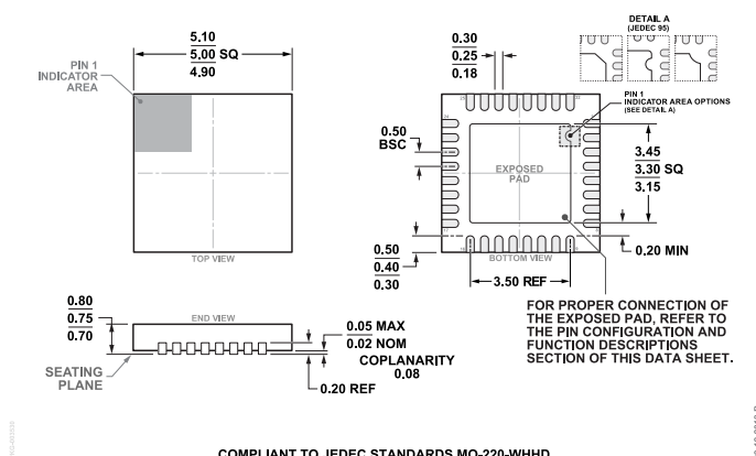
Figure 43. 32-Lead Lead Frame Chip Scale Package [LFCSP] 5 mm x 5 mm Body and 0.75 mm Package Height (CP-32-13) Dimensions shown in millimeters
