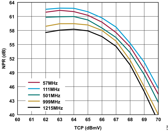
Figure 26. NPR vs. TCP Over Frequency, 0 dB Tilt, V_{DD} = 8.0\text{ V}
