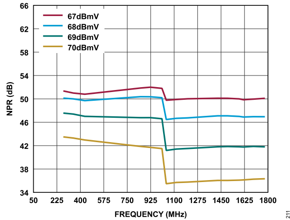
Figure 11. NPR vs. Frequency Over TCP, 10 dB Tilt, V_{DD} = 8.0\text{ V}
