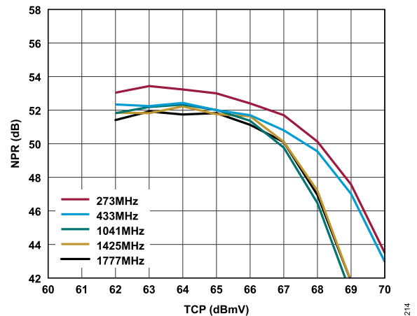
Figure 14. NPR vs. TCP Over Frequency, 10 dB Tilt, V_{DD} = 8.0\text{ V}
