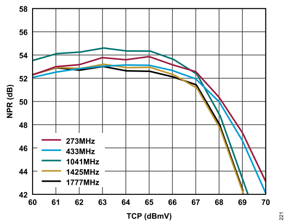
Figure 21. NPR vs. TCP Over Frequency, 10 dB Tilt, No Offset at 1026 MHz, V_{DD} = 8.0\text{ V}
