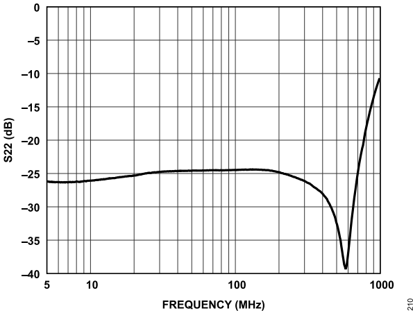
Figure 10. Upstream S22 vs. Frequency Over Temperature
