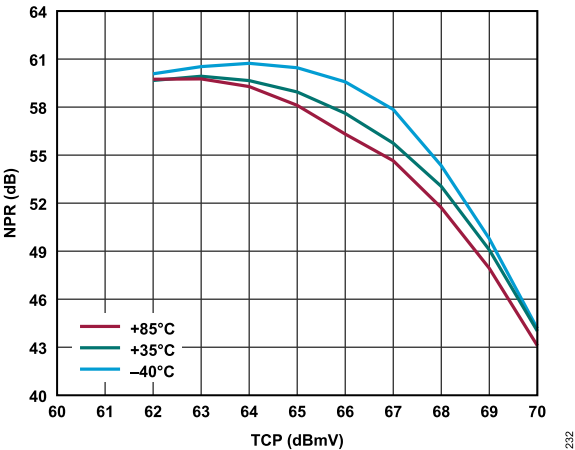
Figure 34. NPR vs. TCP Over Temperature, Worst Case Frequency, 10 dB Tilt, V_{DD} = 8.0\text{ V}
