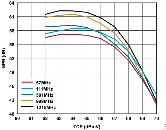
Figure 25. NPR vs. TCP Over Frequency, 10 dB Tilt, V_{DD} = 8.0\text{ V}
