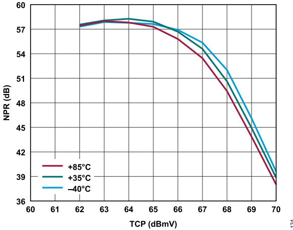
Figure 24. NPR vs. TCP Over Temperature, Worst Case Frequency, 0 dB Tilt, V_{DD} = 8.0\text{ V}
