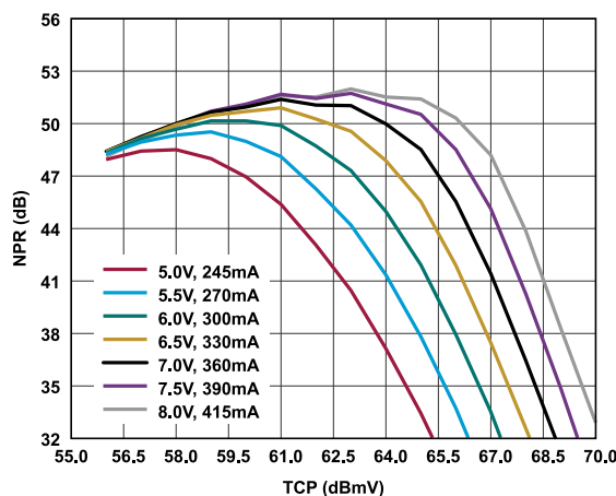
Figure 19. NPR vs. TCP Over V_{DD} and I_{DD} , Worst Case Frequency, 10 dB Tilt, R_{BIAS} = 50 \Omega
