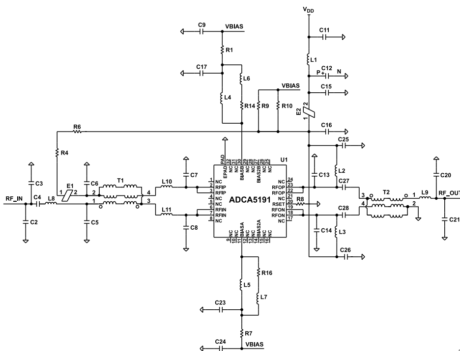
Figure 39. Suggested Downstream Cable TV (CATV) Application Circuit
