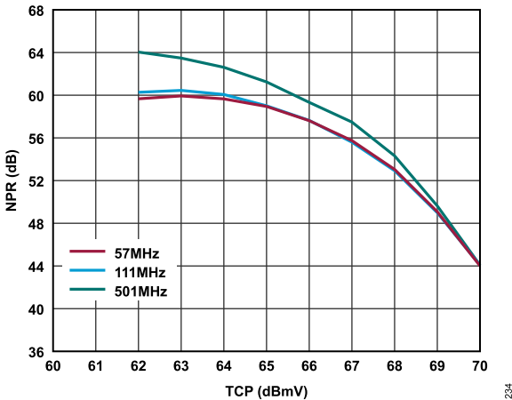
Figure 36. NPR vs. TCP Over Frequency, 10 dB Tilt, V_{DD} = 8.0\text{ V}
