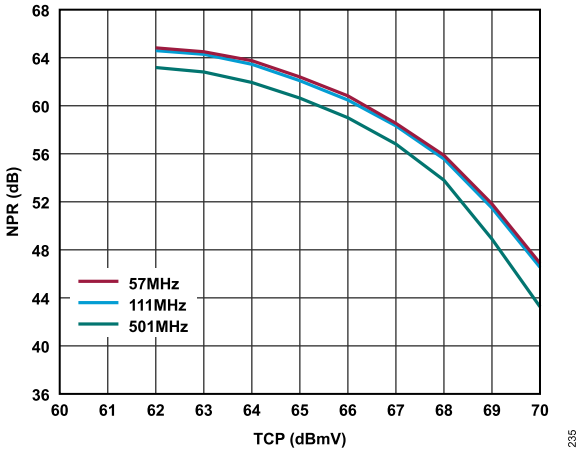
Figure 37. NPR vs. TCP Over Frequency, 0 dB Tilt, V_{DD} = 8.0\text{ V}
