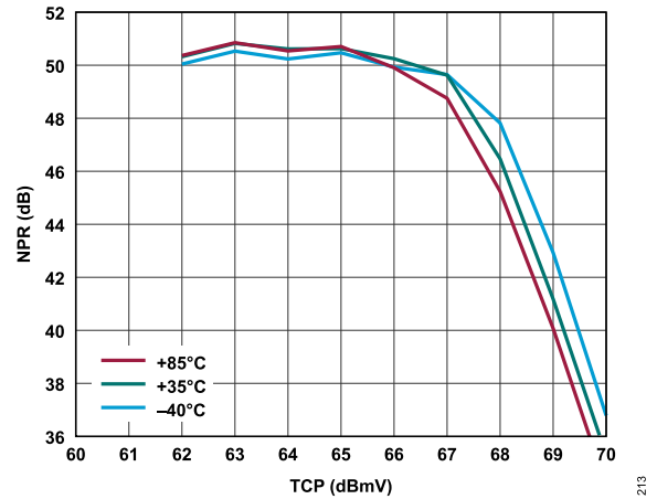
Figure 13. NPR vs. TCP Over Temperature, Worst Case Frequency, 10 dB Tilt, V_{DD} = 8.0\text{ V}
