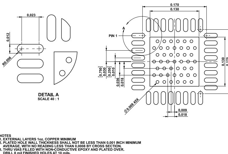
Figure 38. Recommended PCB Layout (Dimensions Shown in Inches)
