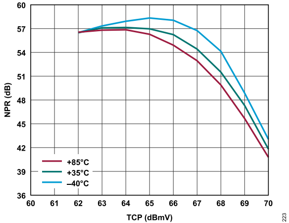
Figure 23. NPR vs. TCP Over Temperature, Worst Case Frequency, 10 dB Tilt, V_{DD} = 8.0\text{ V}
