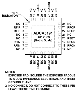
Figure 2. Pin Configuration
