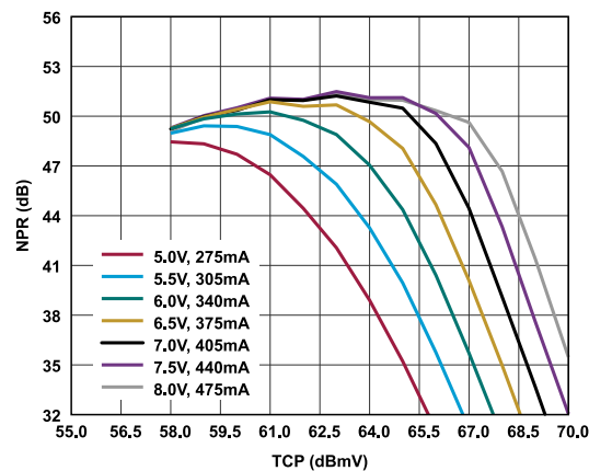
Figure 18. NPR vs. TCP Over V_{DD} and I_{DD} , Worst Case Frequency, 10 dB Tilt, R_{BIAS} = 33 \Omega
