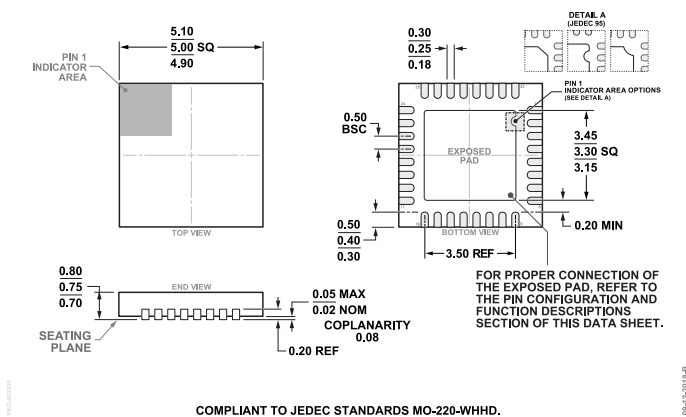
Figure 35. 32-Lead Lead Frame Chip Scale Package [LFCSP] 5 mm x 5 mm Body and 0.75 mm Package Height (CP-32-13) Dimensions shown in millimeters
