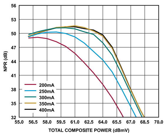
Figure 16. NPR vs. Total Composite Power Over Current, Worst Case Frequency, 10 dB Tilt, V_{DD} = 6.0 V
