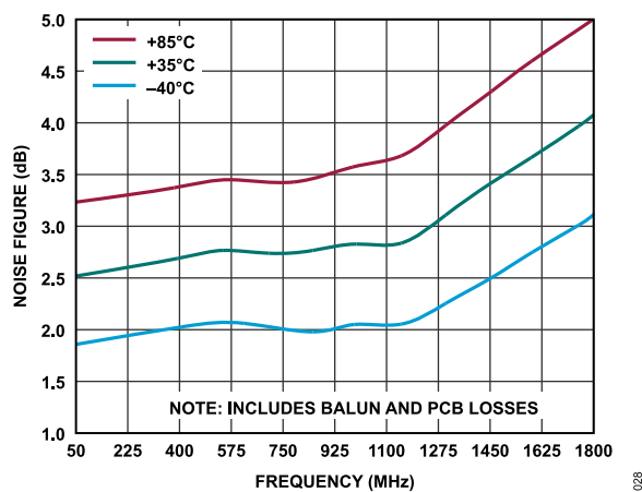
Figure 28. Noise Figure vs. Frequency Over Temperature, V_{DD} = 5.0\text{ V} , I_{DD} = 250\text{ mA}
