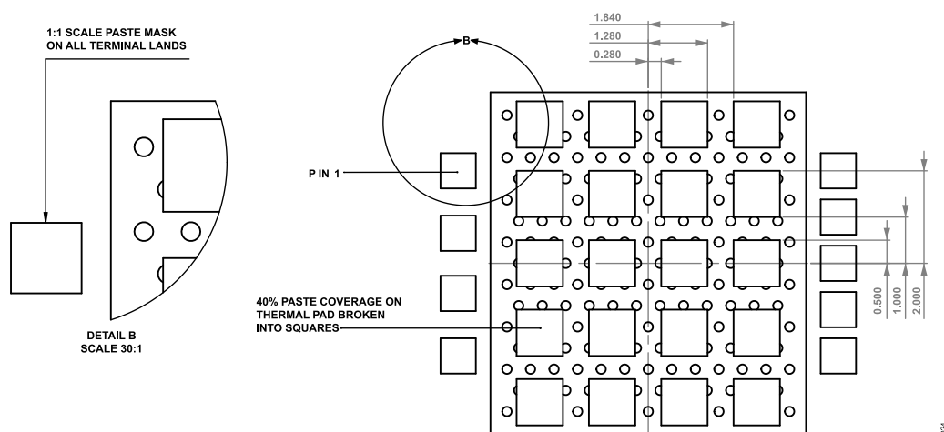
Figure 23. Recommended Solder Pattern (Dimensions Shown in Millimeters)
