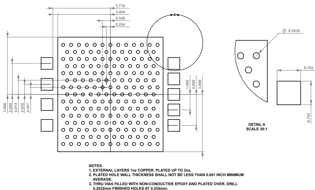
Figure 22. Recommended PCB Layout (Dimensions Shown in Millimeters)
