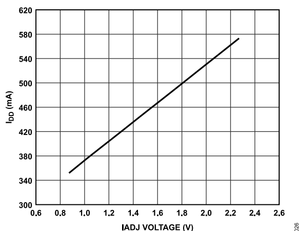
Figure 25. I_{DD} vs. IADJ Voltage over V_{DD}
