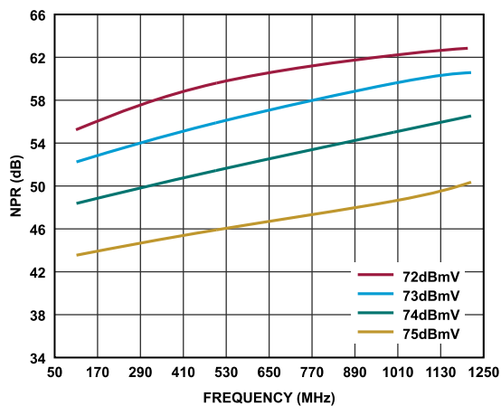
Figure 13. NPR vs. Frequency over TCP, 13 dB Tilt
