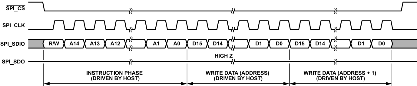
Figure 9. Basic 4-Wire Write Operation
