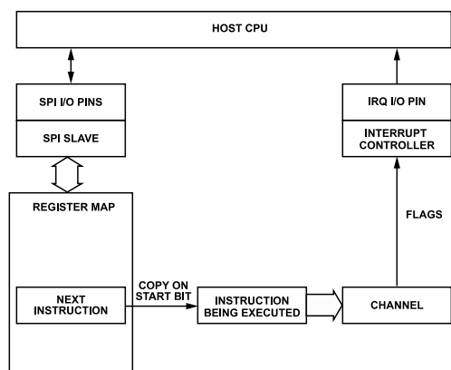
Figure 5. Manual Sequencing Mode
