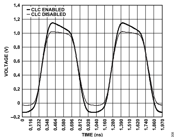
Figure 8. V_{Hx} = 2.0\text{ V} , V_{Lx} = 0.0\text{ V} , 1.0\text{ GHz} Waveform, CLC Disabled and Enabled
