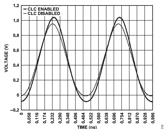
Figure 7. V_{Hx} = 2.0\text{ V} , V_{Lx} = 0.0\text{ V} , 2.0\text{ GHz} Waveform, CLC Disabled and Enabled
