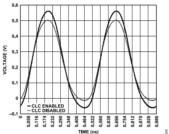
Figure 11. V_{Hx} = 1.0\text{ V} , V_{Lx} = 0.0\text{ V} , 2.0 GHz Waveform, CLC Disabled and Enabled
