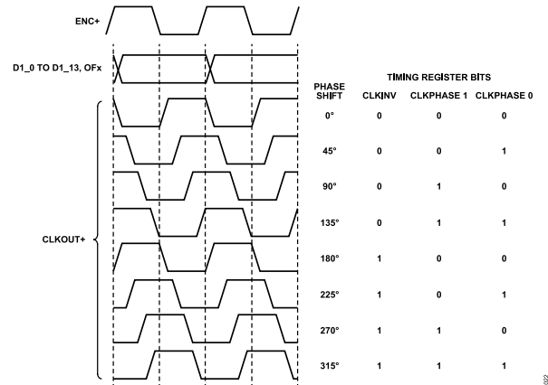
Figure 30. Phase Shifting CLKOUT+
