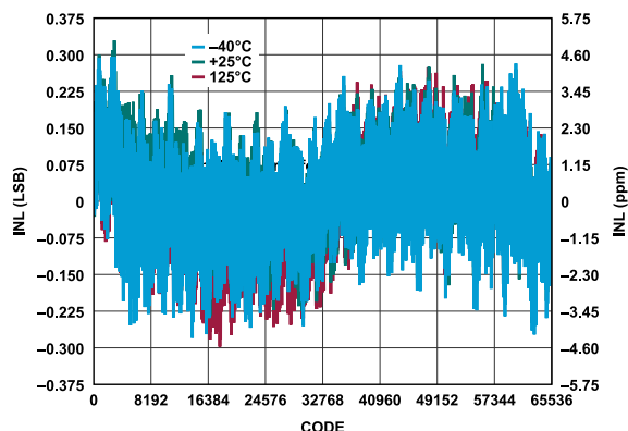
Figure 5. INL vs. Code for Various Temperatures, V_{REF} = 5\text{ V} , G = 0.454
