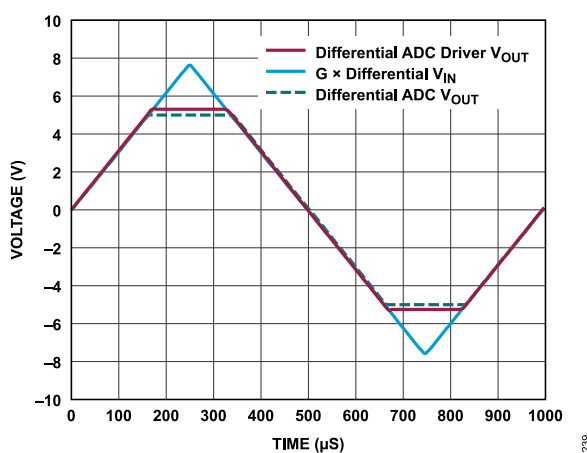
Figure 39. Output Drive Recovery, f_{IN} = 1 kHz
