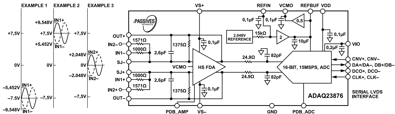
Figure 73. ADAQ23876 Differential Input Configuration with Gain = 0.87, \pm 4.096 V Input Range
