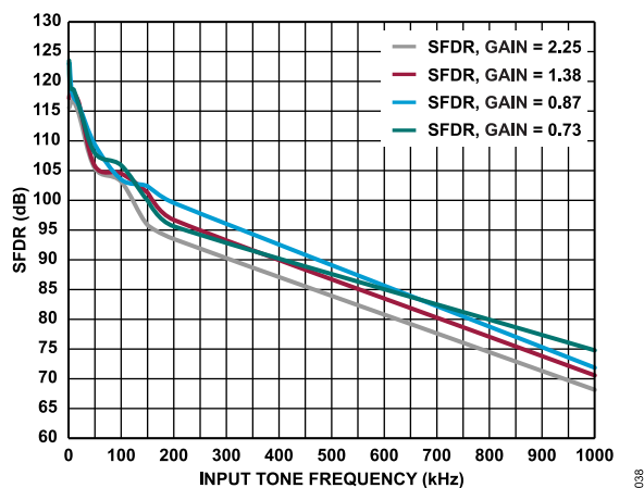
Figure 38. SFDR vs. Input Tone Frequency, Gain = 0.73, Gain = 0.87, Gain = 1.38, and Gain = 2.25
