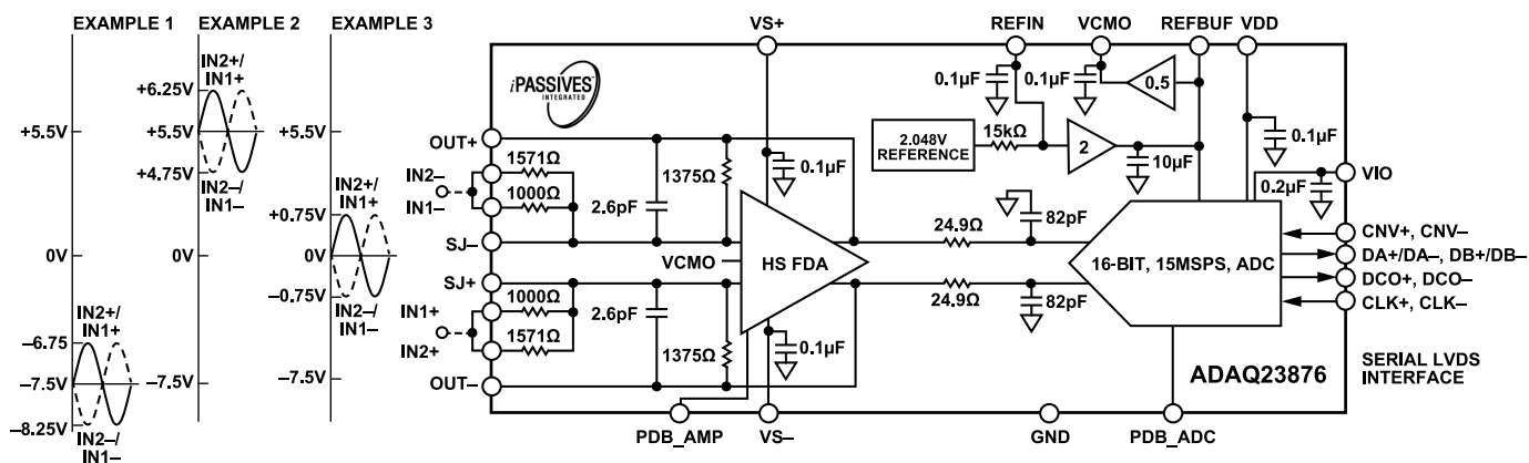
Figure 75. ADAQ23876 Differential Input Configuration with Gain = 2.25, \pm 1.5 V Input Range
