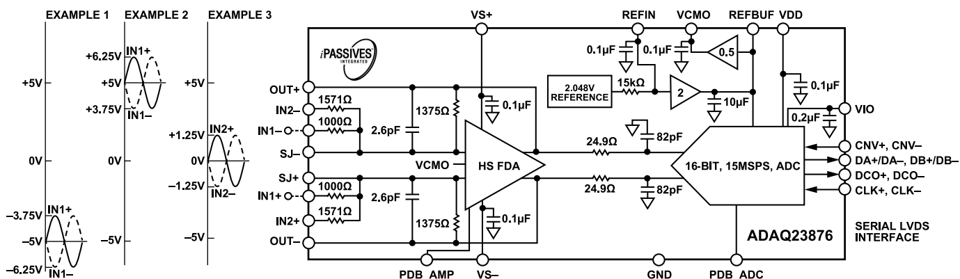
Figure 74. ADAQ23876 Differential Input Configuration with Gain = 1.38, \pm 2.5 V Input Range
