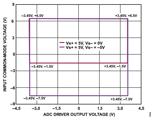
Figure 63. Input Common-Mode Voltage vs. ADC Driver Output Voltage, Gain = 1.38, \pm 2.5 V Differential Input
