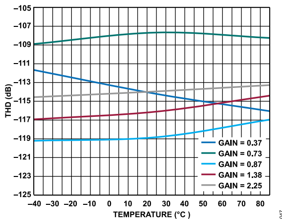
Figure 47. THD vs. Temperature, Gain, f_{IN} = 1 kHz,
