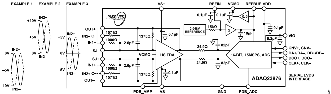
Figure 71. ADAQ23876 Differential Input Configuration with Gain = 0.37, ±10 V Input Range
