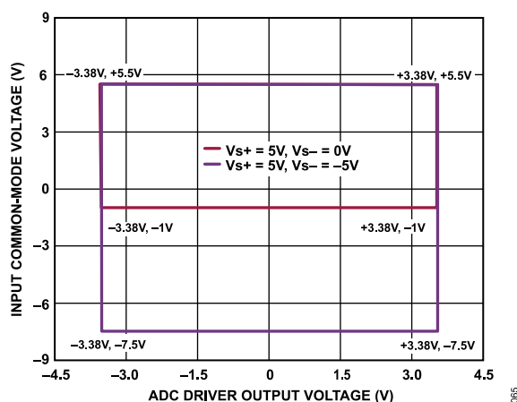
Figure 64. Input Common-Mode Voltage vs. ADC Driver Output Voltage, Gain = 2.25, \pm 1.5 V Differential Input
