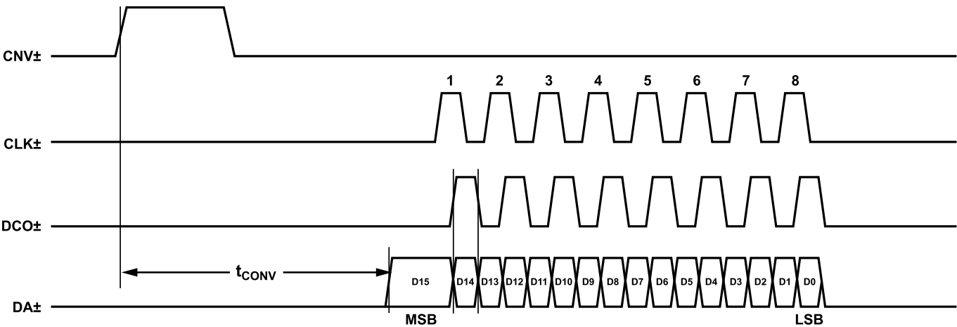
Figure 84. Timing Diagram for a Single Conversion in One-Lane Mode
