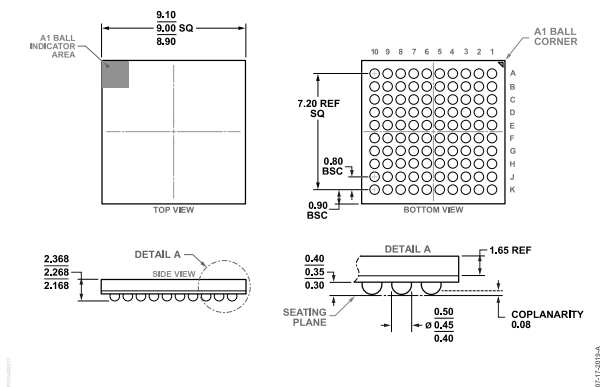
Figure 89. 100-Ball Chip Scale Package Ball Grid Array [CSP_BGA] (BC-100-7) Dimensions shown in millimeters
