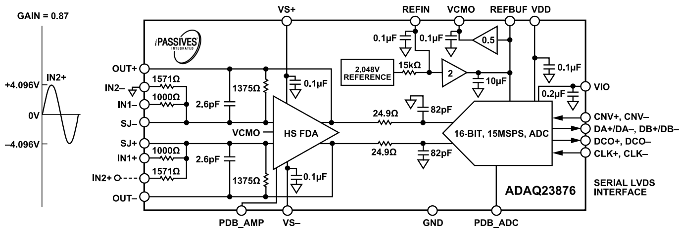
Figure 78. ADAQ23876 Single-Ended Input Configuration with Gain = 0.87
