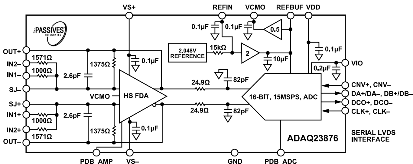
Figure 69. ADAQ23876 \mu Module Simplified Block Diagram
