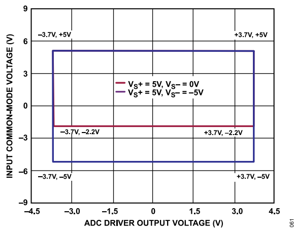
Figure 60. Input Common-Mode Voltage vs. ADC Driver Output Voltage, Gain = 0.37, \pm 10 V Differential Input
