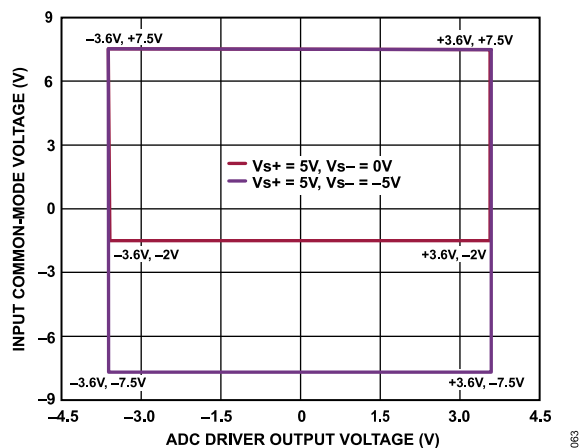
Figure 62. Input Common-Mode Voltage vs. ADC Driver Output Voltage, Gain = 0.87, \pm 4.096 V Differential Input
