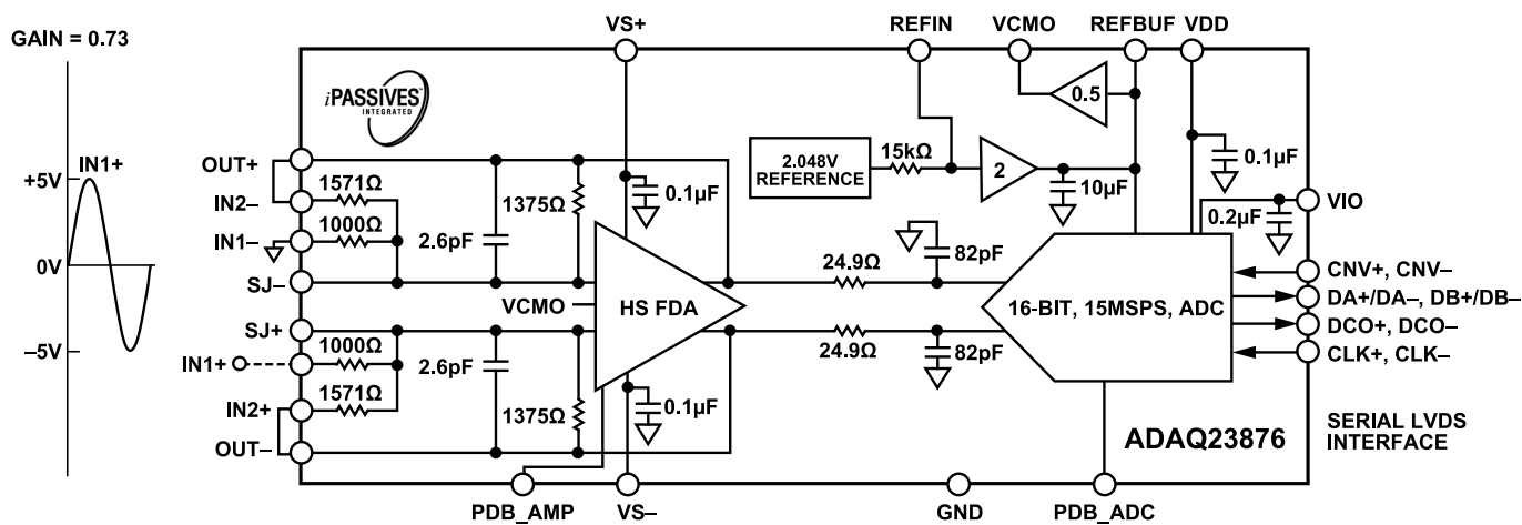
Figure 77. ADAQ23876 Single-Ended Input Configuration with Gain = 0.73
