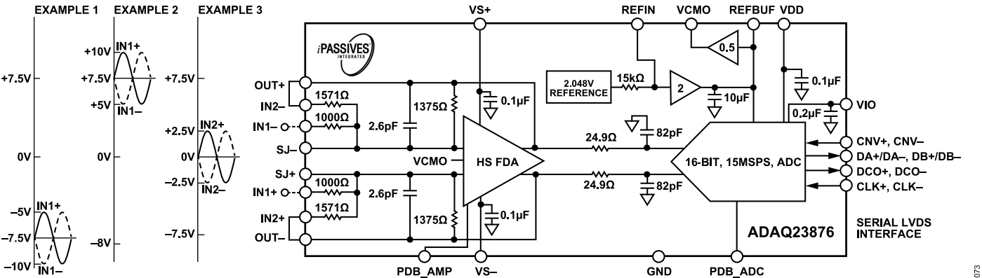
Figure 72. ADAQ23876 Differential Input Configuration with Gain = 0.73, ±5 V Input Range
