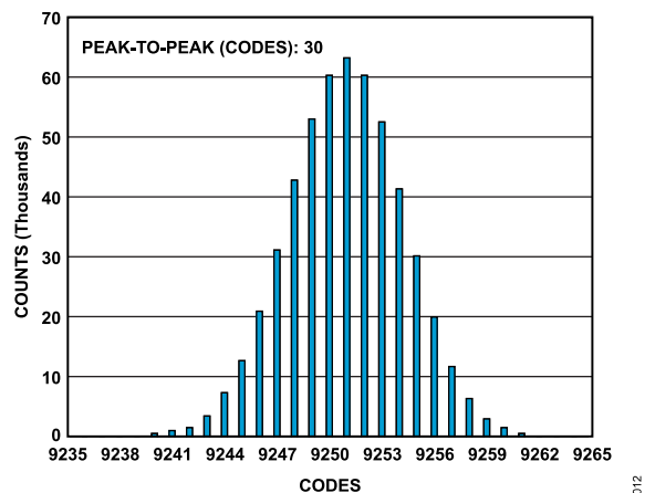
Figure 12. Histogram of a DC Input at the Code Transition
