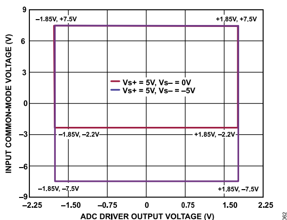
Figure 61. Input Common-Mode Voltage vs. ADC Driver Output Voltage, Gain = 0.73, \pm 5 V Differential Input
