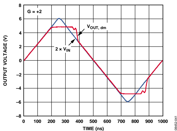
Figure 43. Output Overdrive Recovery, G = 2
