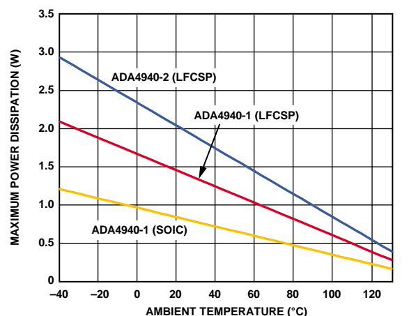
Figure 3. Maximum Safe Power Dissipation vs. Ambient Temperature
