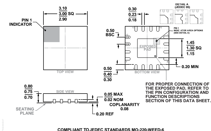
Figure 77. 16-Lead Lead Frame Chip Scale Package [LFCSP] 3 mm × 3 mm Body and 0.75 mm Package Height (CP-16-21)
