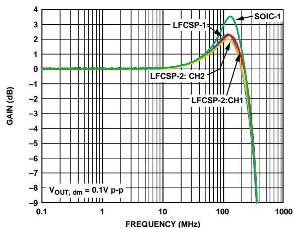
Figure 13. Small Signal Frequency Response for Various Packages
