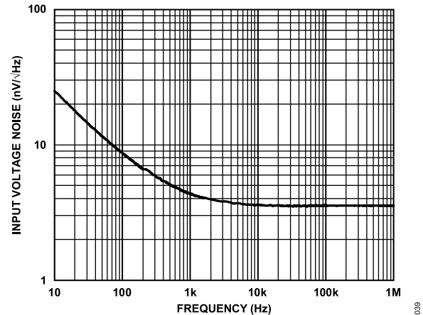
Figure 38. Voltage Noise Spectral Density, Referred to Input
