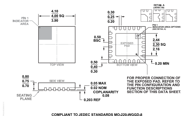
Figure 70. 24-Lead Lead Frame Chip Scale Package [LFCSP] 4 mm x 4 mm Body and 0.75 mm Package Height (CP-24-14) Dimensions shown in millimeters
