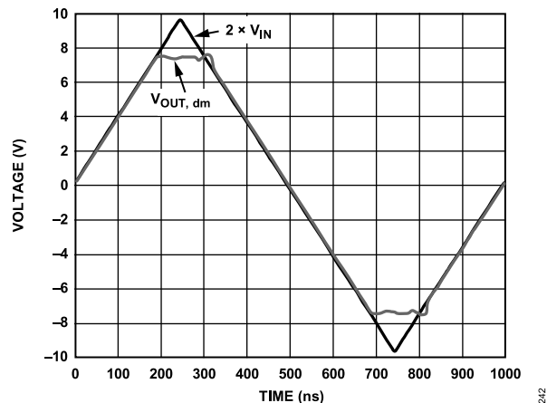
Figure 41. Overdrive Recovery, G = 2
