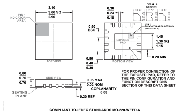
Figure 69. 16-Lead Lead Frame Chip Scale Package [LFCSP] 3 mm x 3 mm Body and 0.75 mm Package Height (CP-16-21) Dimensions shown in millimeters
