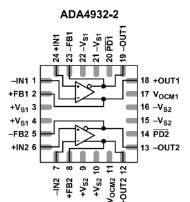
Figure 2. ADA4932-2
