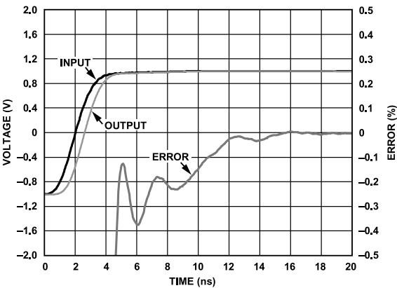
Figure 48. Settling Time
