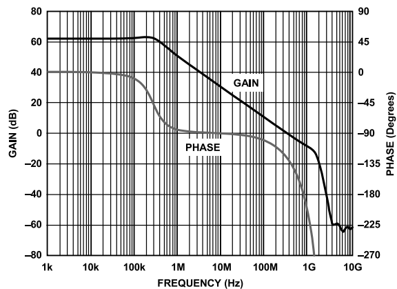
Figure 39. Open-Loop Gain and Phase vs. Frequency
