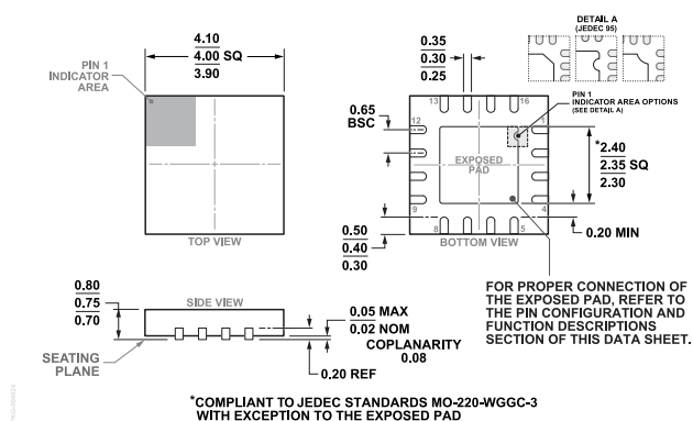
Figure 108. 16-Lead Lead Frame Chip Scale Package [LFCSF] 4 mm x 4 mm Body and 0.75 mm Package Height (CP-16-20) Dimensions shown in millimeters
