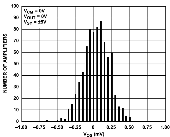
Figure 10. Input Offset Voltage ( V_{OS} ) Distribution, V_{SY} = \pm 5\text{ V}
