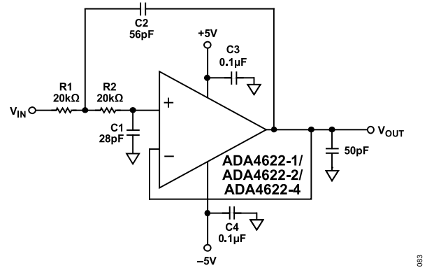
Figure 92. Second-Order, Butterworth, Low-Pass Filter
