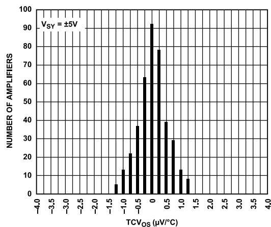
Figure 13. Input Offset Voltage Drift ( TCV_{OS} ) Distribution ( -40^\circ\text{C} to +125^\circ\text{C} ), V_{SY} = \pm 5\text{ V}
