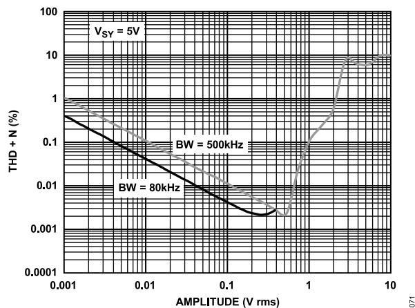
Figure 75. THD + N vs. Amplitude, V_{SY} = 5\text{ V}
