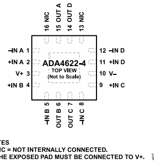
Figure 7. 16-Lead LFCSP Pin Configuration, ADA4622-4
