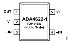
Figure 2. 5-Lead SOT-23 Pin Configuration, ADA4622-1
