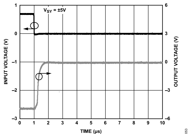
Figure 57. Negative Overload Recovery, A_V = -10 , V_{SY} = \pm 5\text{ V}
