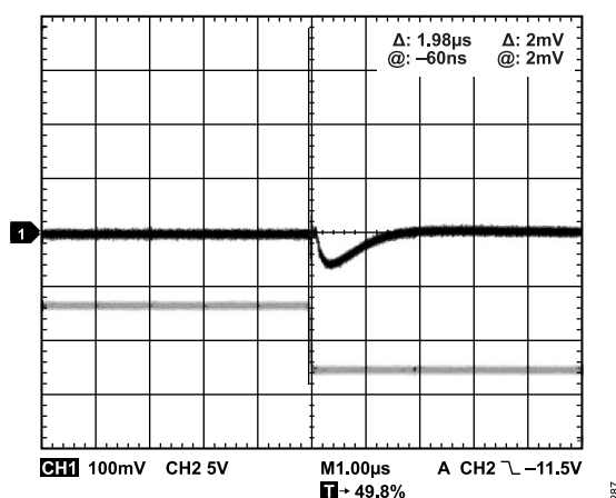
Figure 89. Shutdown Response when Toggling the \overline{\text{DISABLE}} Input
