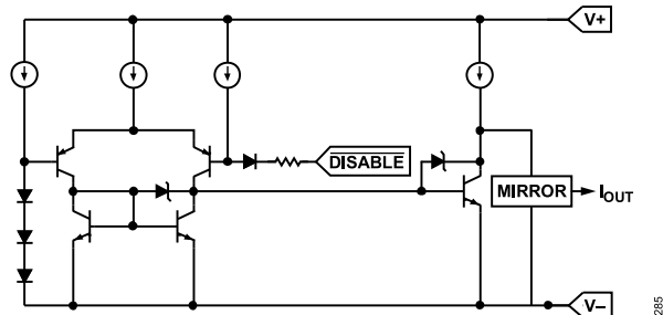
Figure 87. Simplified Circuit for the \overline{\text{DISABLE}} Input
