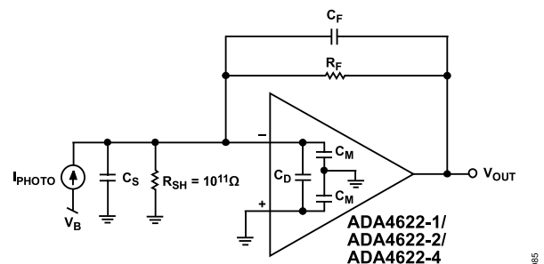
Figure 94. Wideband Photodiode Preamplifier
