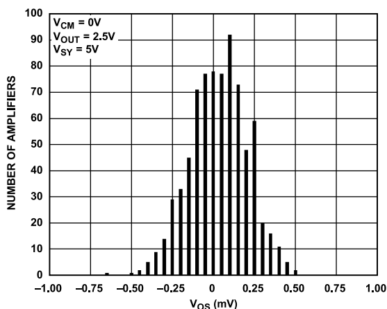
Figure 11. Input Offset Voltage ( V_{OS} ) Distribution, V_{SY} = 5\text{ V}
