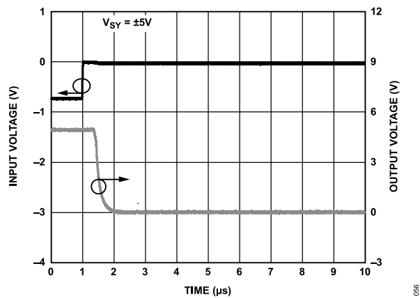
Figure 60. Positive Overload Recovery, A_V = -10 , V_{SY} = \pm 5\text{ V}
