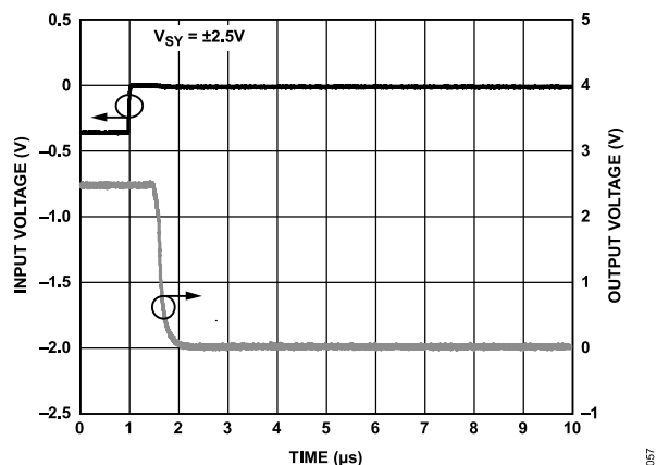
Figure 61. Positive Overload Recovery, A_V = -10 , V_{SY} = \pm 2.5\text{ V}
