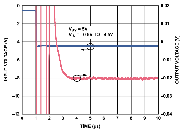
Figure 67. Negative Settling Time, A_V = -10 , V_{SY} = 5\text{ V}
