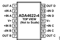
Figure 8. 14-Lead SOIC_N Pin Configuration, ADA4622-4
