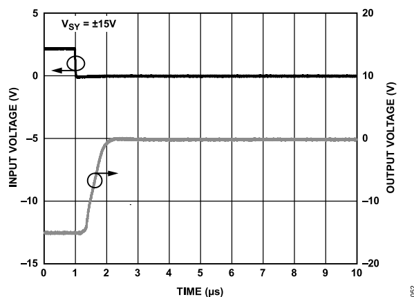
Figure 56. Negative Overload Recovery, A_V = -10 , V_{SY} = \pm 15\text{ V}
