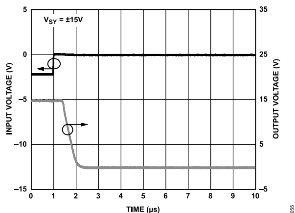
Figure 59. Positive Overload Recovery, A_V = -10 , V_{SY} = \pm 15\text{ V}
