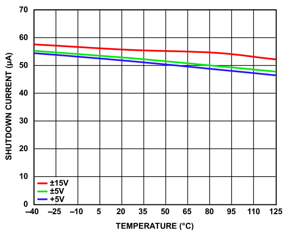
Figure 79. Shutdown Current vs. Temperature
