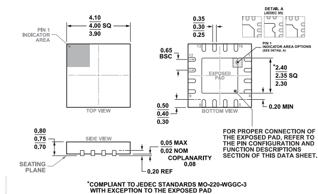
Figure 108. 16-Lead Lead Frame Chip Scale Package [LFCSP] 4 mm x 4 mm Body and 0.75 mm Package Height (CP-16-20) Dimensions shown in millimeters
