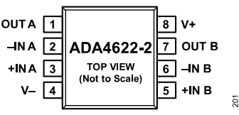
Figure 5. 8-Lead SOIC_N Pin Configuration, ADA4622-2
