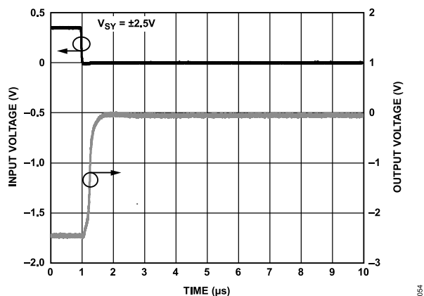
Figure 58. Negative Overload Recovery, A_V = -10 , V_{SY} = \pm 2.5\text{ V}
