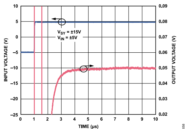
Figure 62. Positive Settling Time, A_V = -10 , V_{SY} = \pm 15\text{ V}
