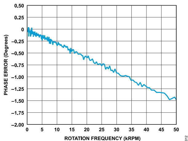
Figure 12. Phase Error vs. Mechanical RPM
