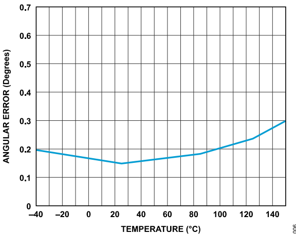
Figure 6. Single Point Calibration Angular Error vs. Temperature
