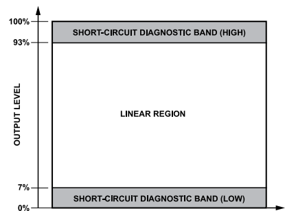
Figure 20. Short-Circuit Diagnostic Band
