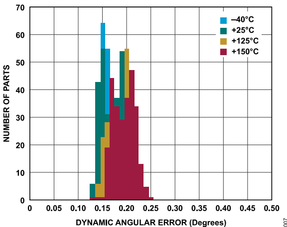
Figure 7. Dynamic Angular Error Histogram
