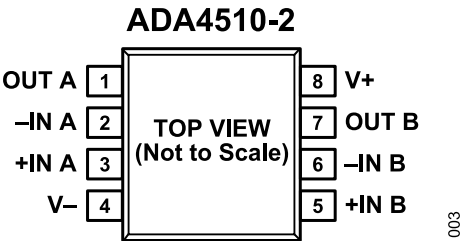
Figure 3. 8-Lead SOIC_N and 8-Lead MSOP Pin Configuration
