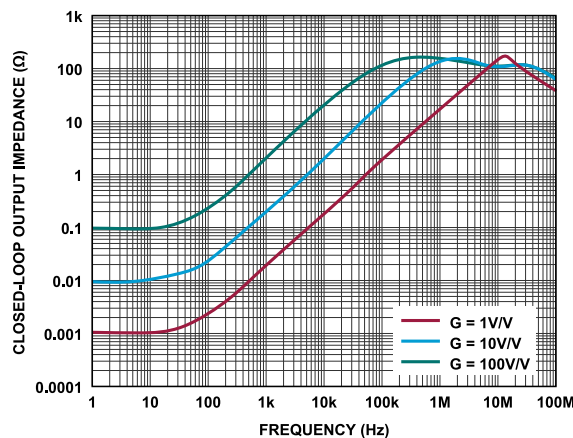
Figure 33. Z_{\text{OUT}} vs. Frequency
