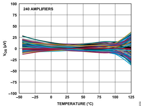
Figure 13. V_{OS} vs. Temperature, SOIC_N
