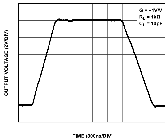
Figure 67. Large Signal Transient Response, G = -1\text{ V/V}
