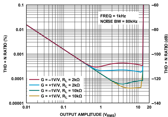
Figure 48. THD Plus Noise (THD + N) Ratio vs. Output Amplitude
