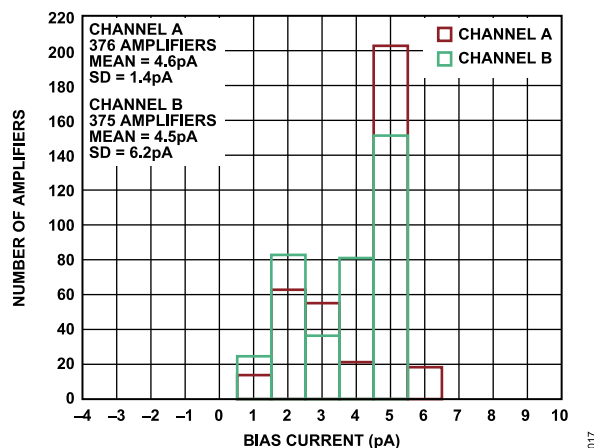
Figure 20. I_B Distribution at -40°C
