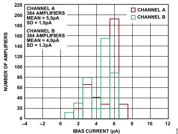
Figure 19. I_B Distribution at 25°C
