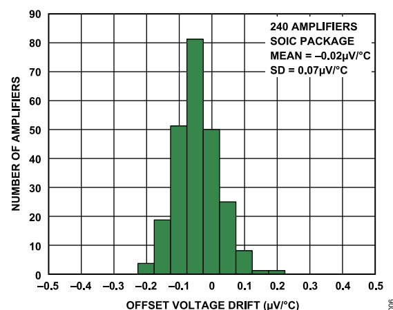
Figure 6. Input Offset Voltage Drift ( TCV_{OS} ) Distribution from 0^\circ\text{C} to +85^\circ\text{C} , SOIC_N
