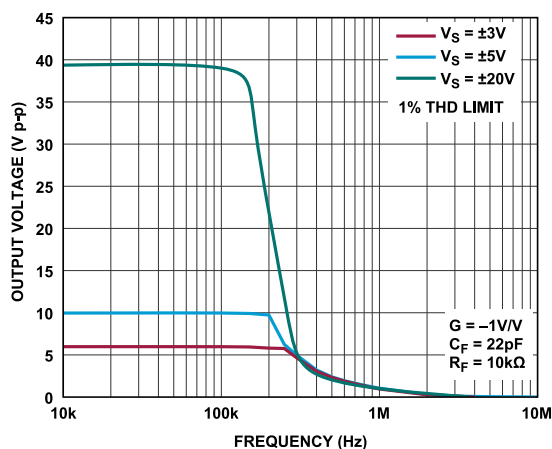
Figure 50. Maximum Undistorted Output Swing vs. Frequency
