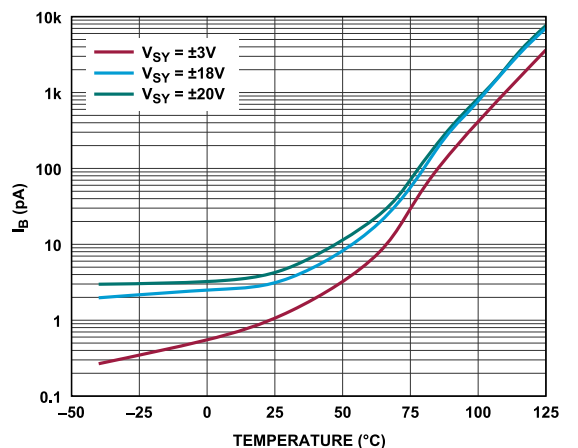
Figure 26. I_B vs. Temperature, SOIC_N
