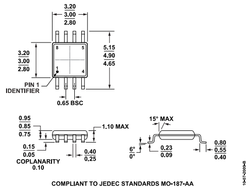
Figure 94. 8-Lead Mini Small Outline Package [MSOP] (RM-8) Dimensions Shown in millimeters
