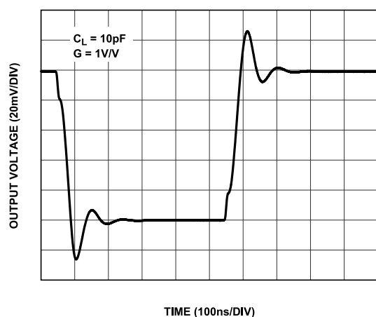
Figure 59. Small Signal Transient Response, G = 1\text{V/V}
