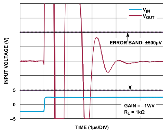
Figure 51. Positive Step Settling Time to 0.01%, V_{OUT} = 5\text{ V}
