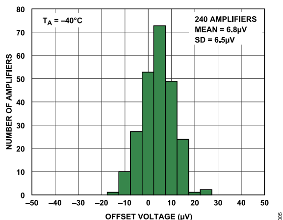
Figure 5. V_{OS} Distribution at -40^\circ\text{C}
