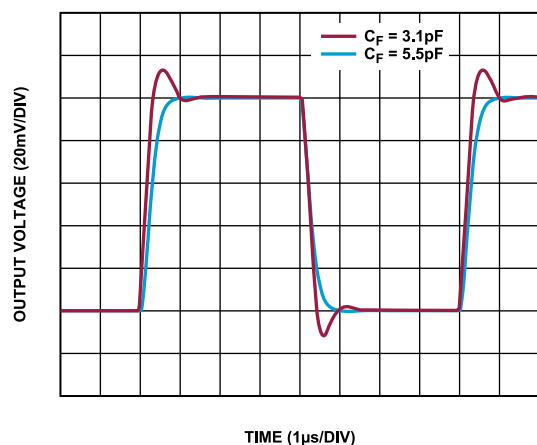
Figure 89. Pulse Response for Various C_F
