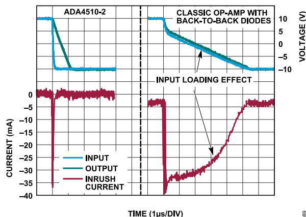
Figure 80. ADA4510-2 Inrush Current Reduction
