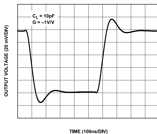
Figure 62. Small Signal Transient Response, G = -1\text{V/V}
