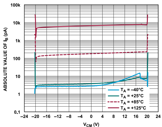
Figure 29. I_B vs. V_{\text{CM}} , Four Temperatures, SOIC_N
