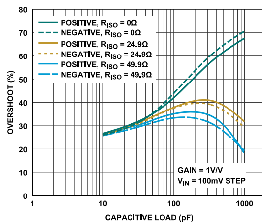
Figure 63. Overshoot vs. Capacitance Load, G = 1\text{V/V}
