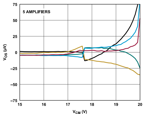
Figure 17. V_{OS} vs. V_{CM} , High V_{CM} Operation
