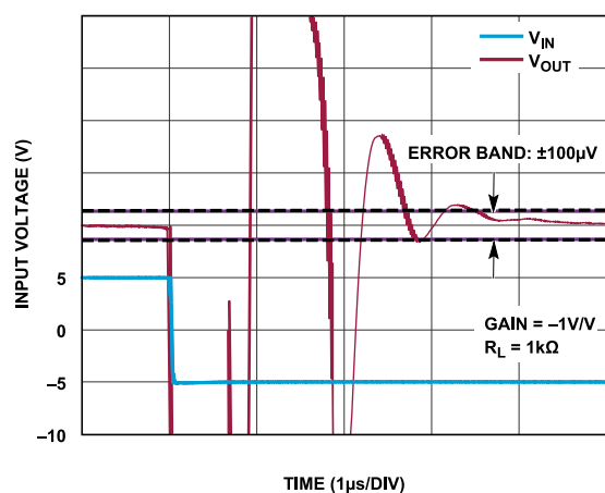
Figure 60. Negative Step Settling Time to 0.001%, V_{OUT} = 10\text{V}
