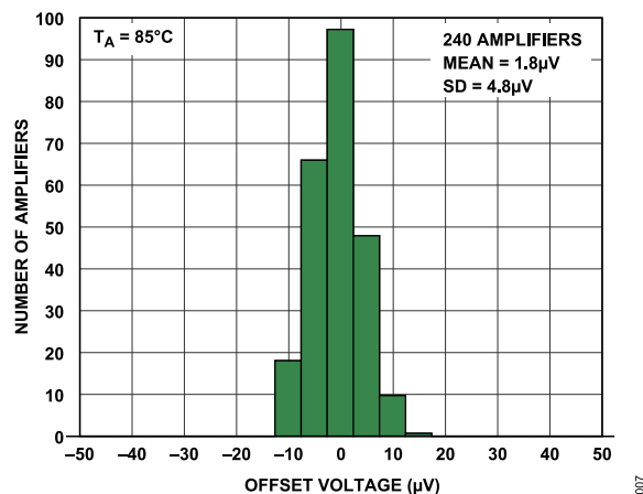
Figure 7. V_{OS} Distribution at 85^\circ\text{C}
