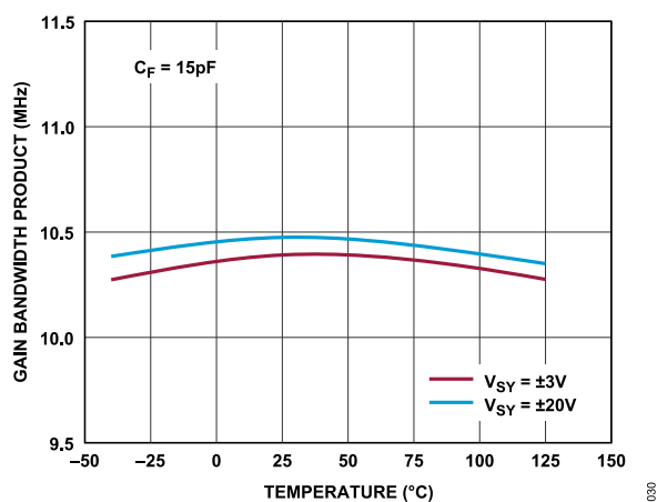
Figure 35. Gain Bandwidth Product vs. Temperature
