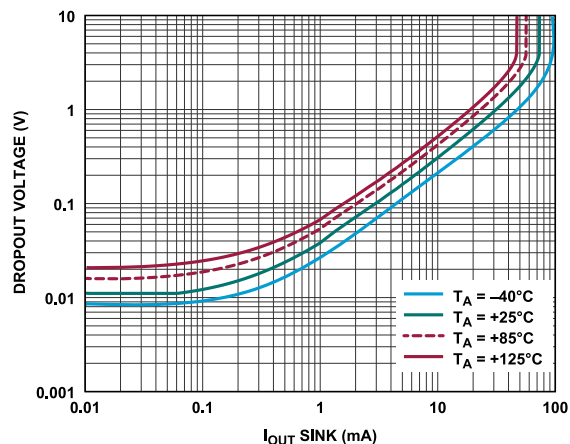
Figure 31. V_{\text{DROP-OUT}}(V_{\text{OUT}} - (V-)) vs. I_{\text{OUT Sink}}
