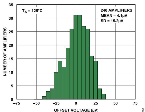
Figure 8. V_{OS} Distribution at 125^\circ\text{C}
