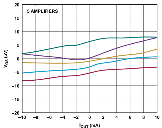
Figure 30. V_{\text{OS}} vs. I_{\text{OUT}}
