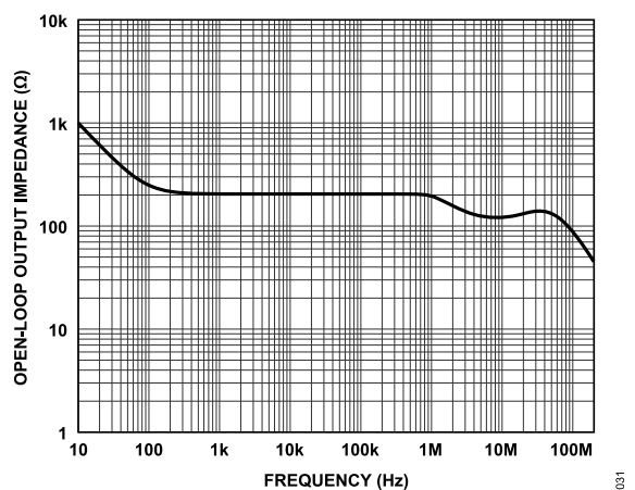
Figure 36. Z_O vs. Frequency
