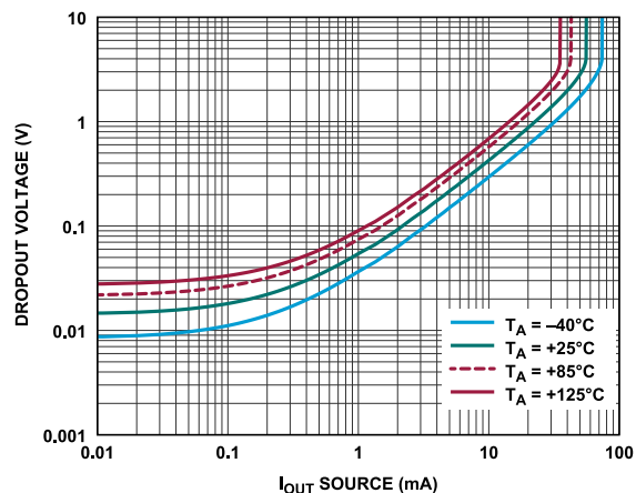
Figure 28. V_{\text{DROP-OUT}}((V+) - V_{\text{OUT}}) vs. I_{\text{OUT Source}}
