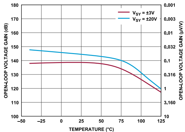
Figure 75. DC Open-Loop Gain vs. Temperature
