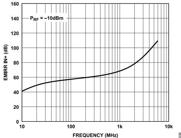
Figure 41. EMIRR IN+ vs. Frequency ( P_{RF} Is RF Power.)
