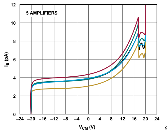
Figure 25. I_B vs. V_{CM}
