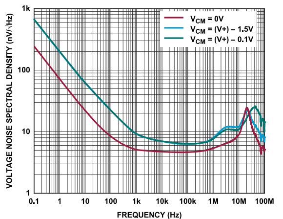
Figure 69. Input Voltage Noise Spectral Density vs. Frequency
