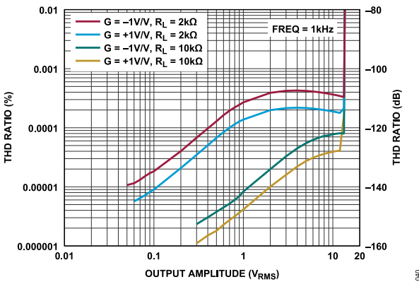
Figure 45. THD Ratio vs. Output Amplitude
