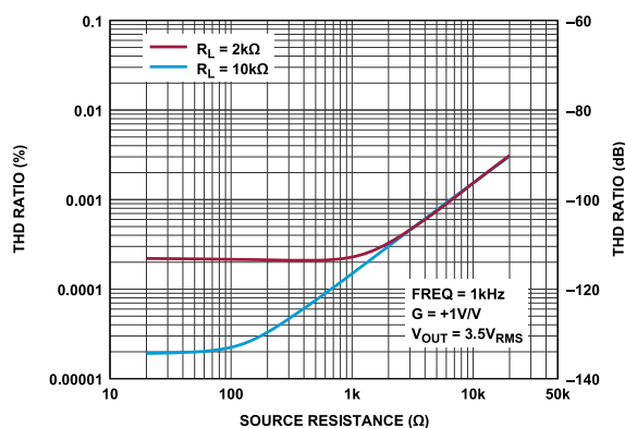
Figure 47. THD Ratio vs. Source Resistance
