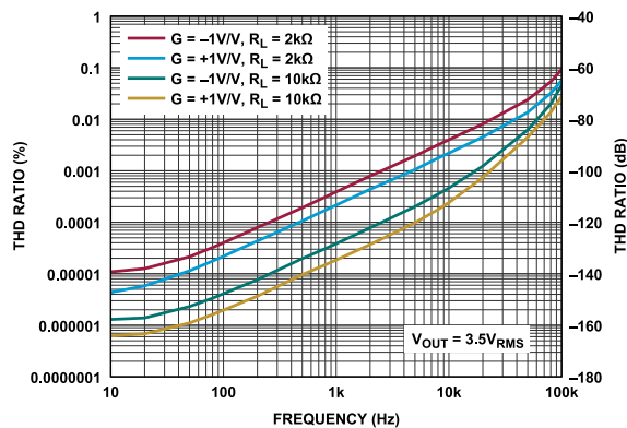
Figure 46. THD Ratio vs. Frequency
