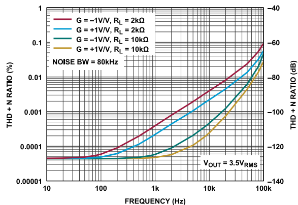
Figure 49. THD + N vs. Frequency
