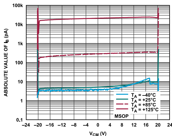
Figure 32. I_B vs. V_{\text{CM}} , Four Temperatures, MSOP
