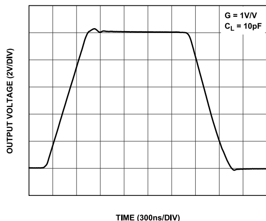
Figure 64. Large Signal Transient Response, G = 1\text{ V/V}
