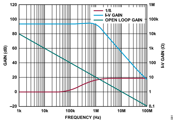
Figure 87. Compensating the TIA, C_F = 3.1 \text{ pF}
