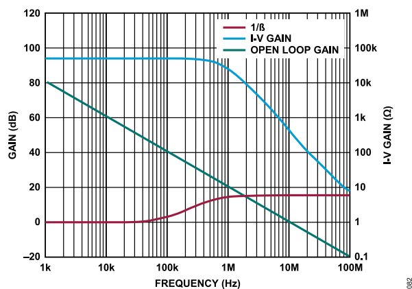
Figure 88. Compensating the TIA, C_F = 5.5 \text{ pF}
