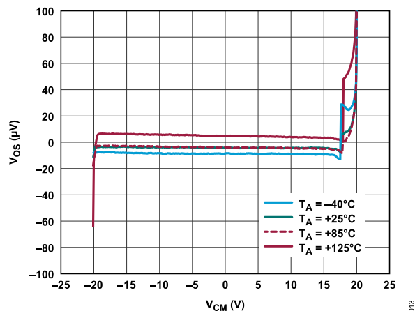
Figure 16. V_{OS} vs. V_{CM} , Four Temperatures
