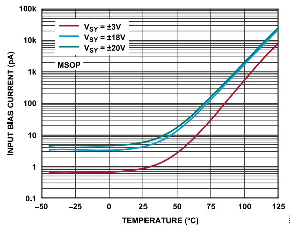
Figure 27. I_B vs. Temperature, MSOP
