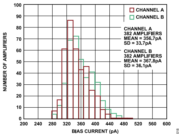
Figure 21. I_B Distribution at 85°C
