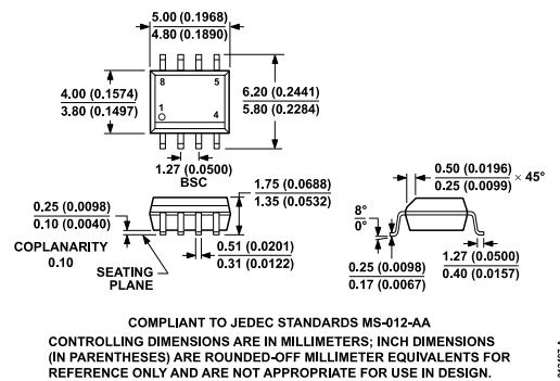
Figure 93. 8-Lead Standard Small Outline Package [SOIC_N] Narrow Body (R-8) Dimensions show in millimeters and (inches)
