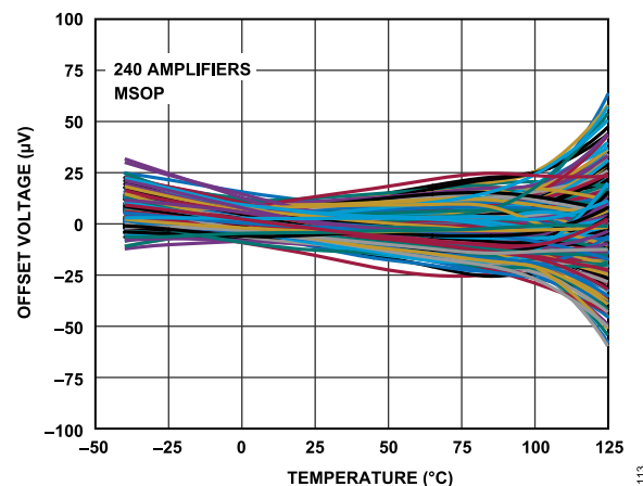
Figure 14. V_{OS} vs. Temperature, MSOP
