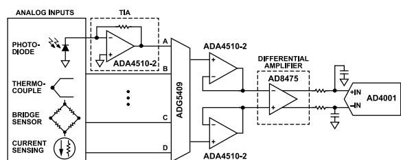
Figure 79. Multiplexed Data Acquisition System
