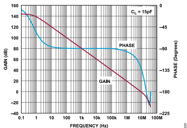
Figure 34. Open-Loop Gain and Phase vs. Frequency
