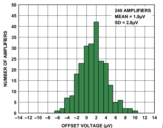
Figure 4. V_{OS} Distribution at 25^\circ\text{C}
