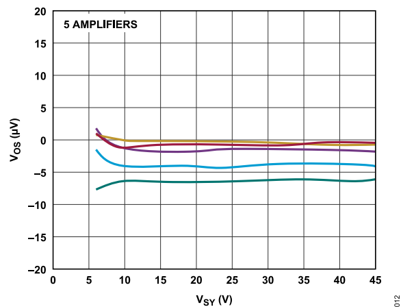
Figure 15. V_{OS} vs. V_{SY}
