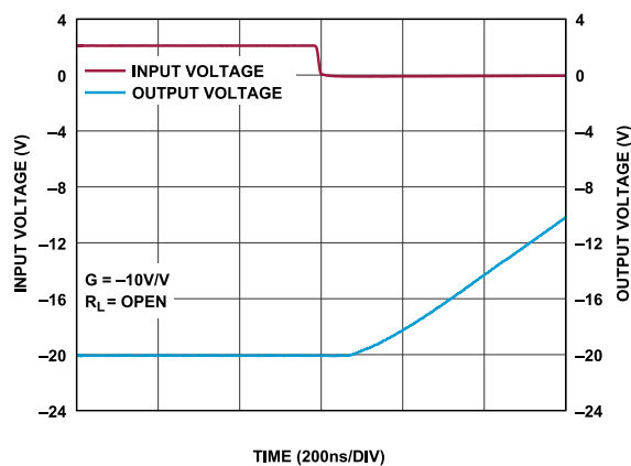
Figure 61. Negative Overload Recovery
