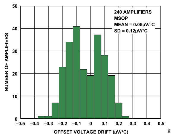
Figure 9. Input Offset Voltage Drift ( TCV_{OS} ) Distribution from 0^\circ\text{C} to +85^\circ\text{C} , MSOP
