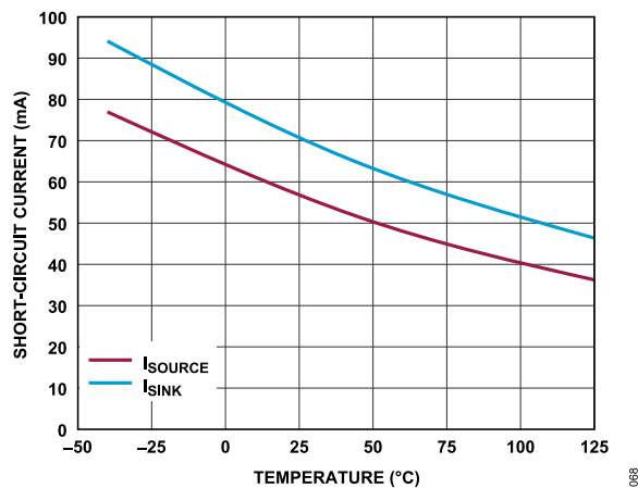
Figure 73. Short-Circuit Output Current vs. Temperature
