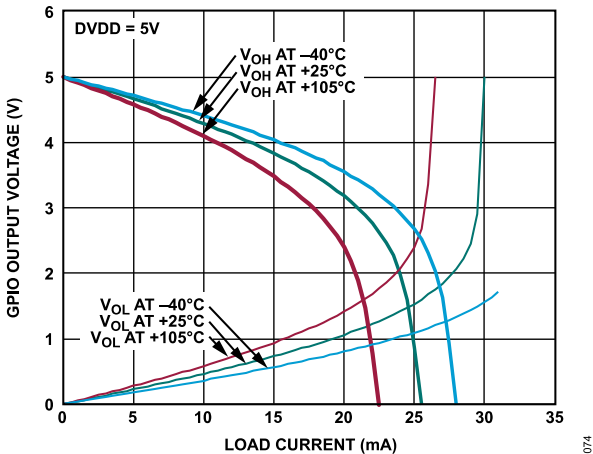
Figure 73. GPIO Output Voltage ( V_{OH}/V_{OL} ) vs. Load Current for Various Temperatures, DVDD = 5\text{V}
