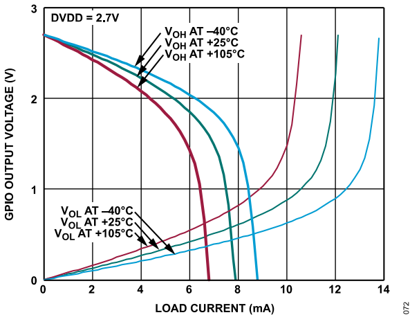
Figure 72. GPIO Output Voltage ( V_{OH}/V_{OL} ) vs. Load Current for Various Temperatures, DVDD = 2.7\text{V}
