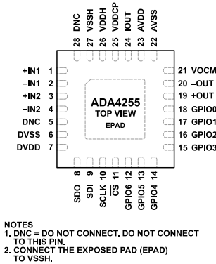
Figure 5. Pin Configuration
