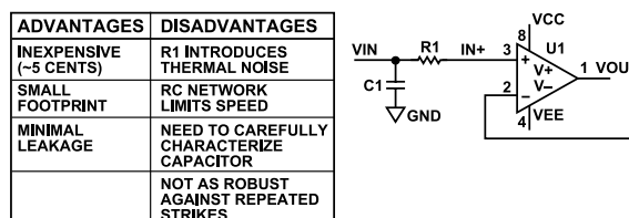
Figure 64. ESD Protection Circuit (RC Network)
