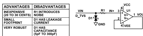
Figure 65. ESD Protection Circuit (R-TVS Network)
