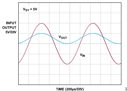
Figure 68. \pm 10 V to 0 V to +5 V Funnel Amplifier, Input and Output Voltages
