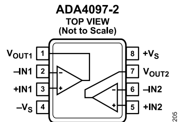
Figure 5. Pin Configuration for ADA4097-2 8-Lead SOIC_N and 8-Lead MSOP
