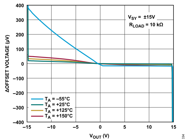
Figure 36. ΔOffset Voltage vs. V_{OUT} Across Various Temperatures
