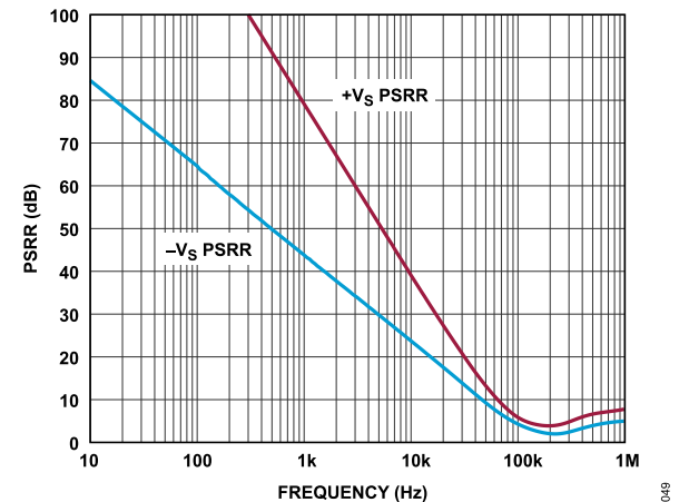
Figure 51. PSRR vs. Frequency
