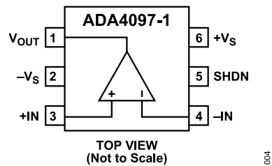
Figure 4. Pin Configuration for the ADA4097-1 6-Lead TSOT
