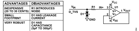
Figure 66. ESD Protection Circuit (R-TVS Network)
