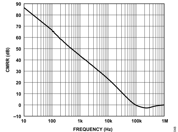
Figure 50. CMRR vs. Frequency
