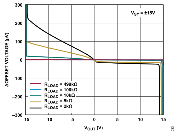
Figure 35. ΔOffset Voltage vs. V_{OUT} Across Various R_{LOAD}
