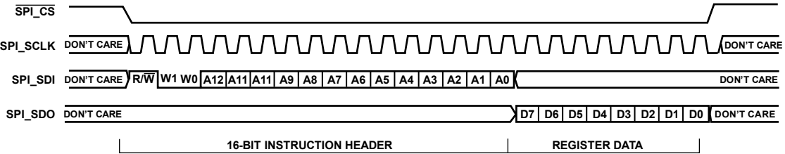
Figure 21. 4-Wire SPI Interface Timing, MSB First Read
