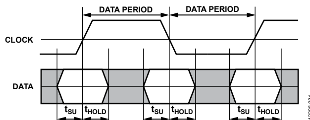
Figure 29. DAC Input LVDS Lane Timing
