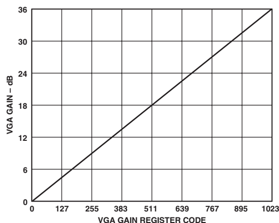
Figure 29. VGA Gain Curve (Gain from PxGA Not Included)
